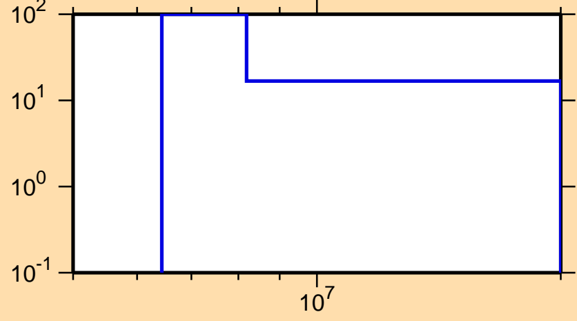
\Delta\sigma/\sigma vs. E for ^{86}\text{Rb}(n,2n)
