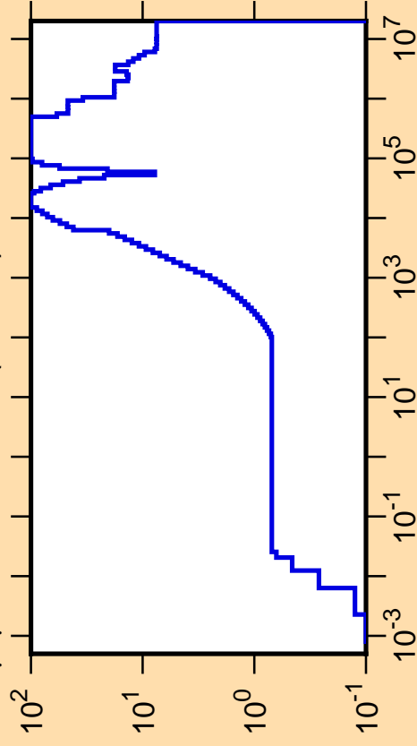
\Delta\mu/\mu vs. E for ^{88}\text{Rb}(\text{mt251})
