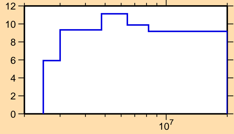
\Delta\sigma/\sigma vs. E for ^{88}\text{Rb}(n,el.)
