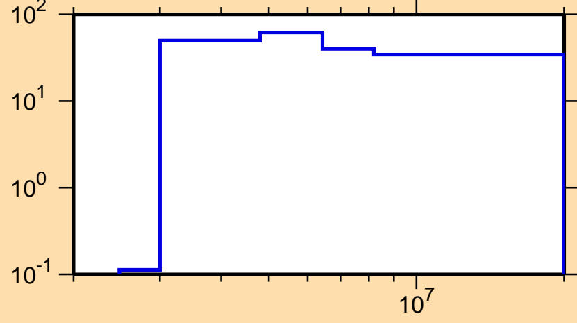
\Delta\sigma/\sigma vs. E for ^{88}\text{Rb}(n,p)
