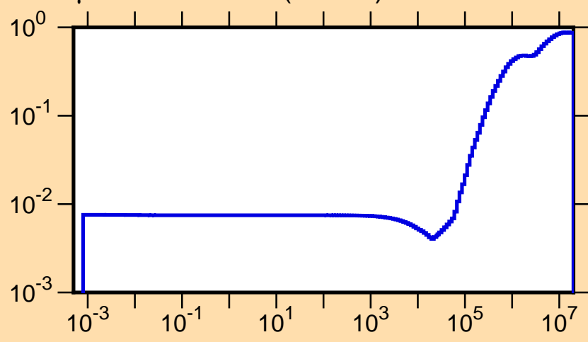
\mu vs. E for ^{89}\text{Rb}(\text{mt251})
