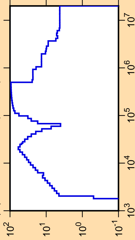
\Delta\mu/\mu vs. E for ^{90}\text{Rb}(\text{mt251})
