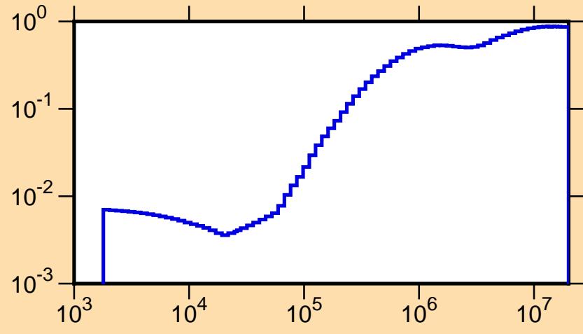
\mu vs. E for ^{90}\text{Rb}(\text{mt251})
