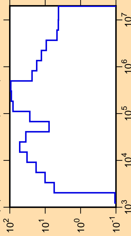
\Delta\mu/\mu vs. E for ^{90}\text{Rb}(\text{mt251})
