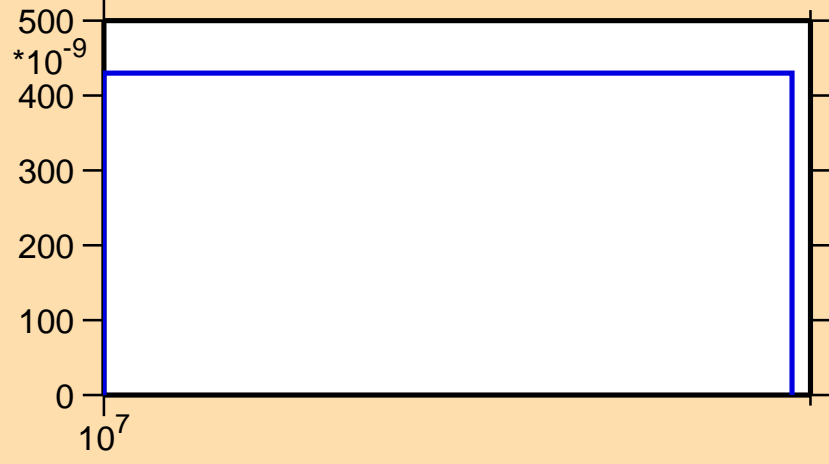
\sigma vs. E for ^{90}\text{Rb}(n,nd)
