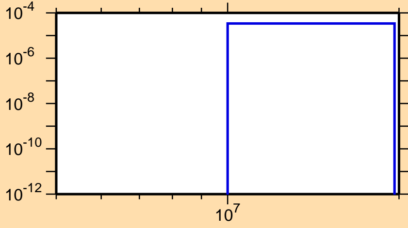
\sigma vs. E for ^{90}\text{Rb}(n,\alpha)
