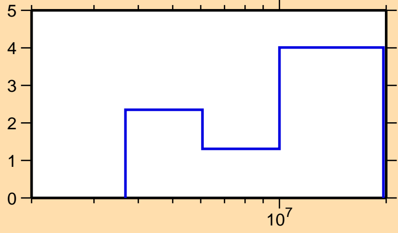
\Delta\sigma/\sigma vs. E for ^{90}\text{Rb}(n,\text{tot.})
