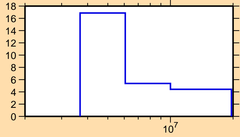
\Delta\sigma/\sigma vs. E for ^{90}\text{Rb}(n,2n)
