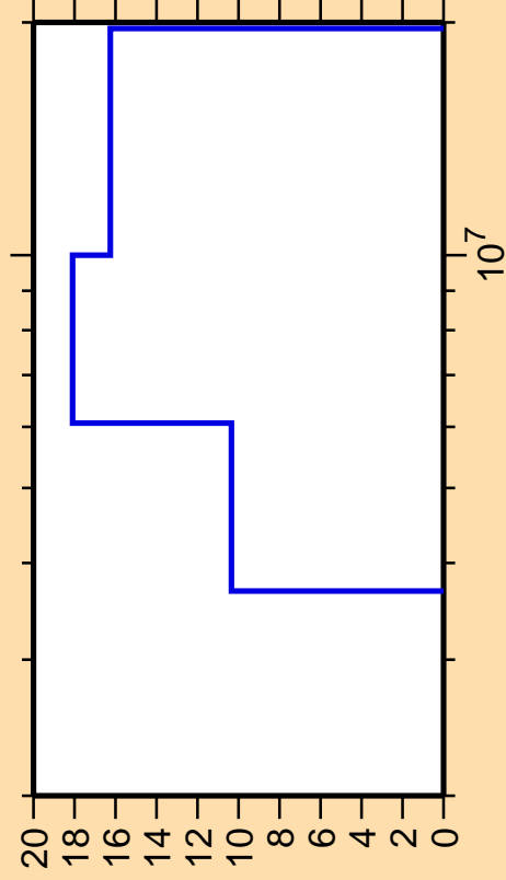
\Delta\sigma/\sigma vs. E for ^{90}\text{Rb}(n,n_1)
