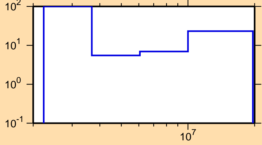
\Delta\sigma/\sigma vs. E for ^{90}\text{Rb}(n,n\text{cont.})
