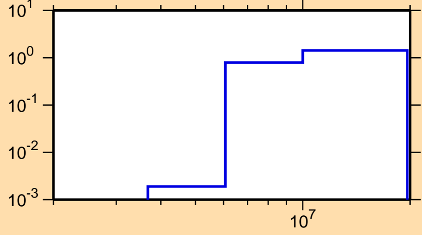
\sigma vs. E for ^{90}\text{Rb}(n,2n)
