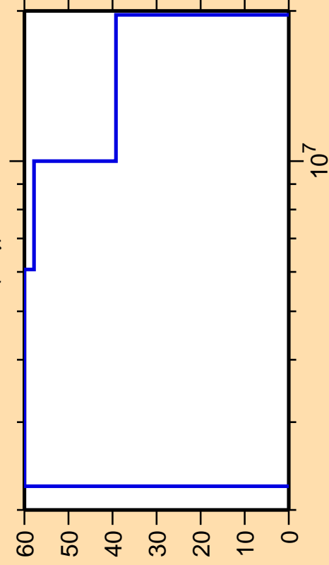
\Delta\sigma/\sigma vs. E for ^{90}\text{Rb}(n,\gamma)
