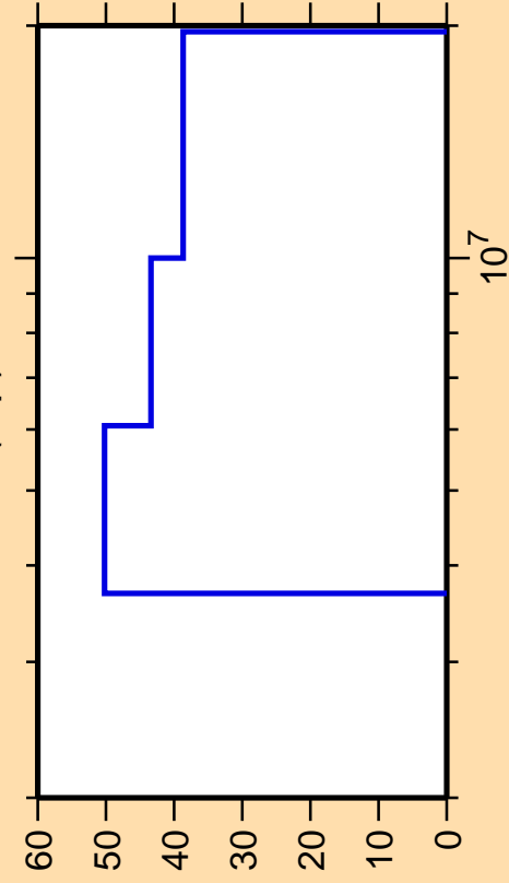
\Delta\sigma/\sigma vs. E for ^{90}\text{Rb}(n,p)
