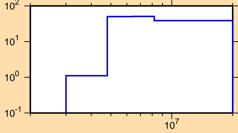
\Delta\sigma/\sigma vs. E for ^{90}\text{Rb}(n,p)
