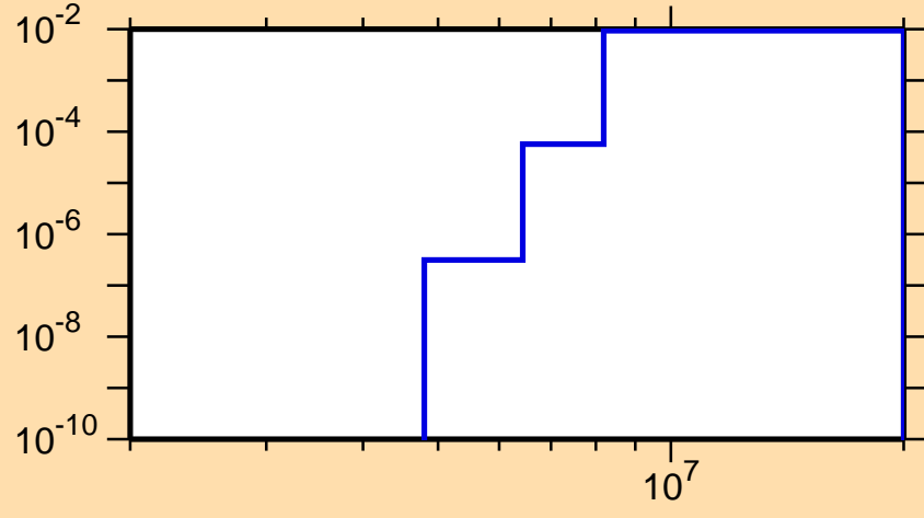
\sigma vs. E for ^{90}\text{Rb}(n,p)
