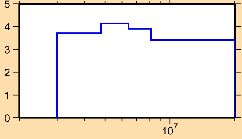
\Delta\sigma/\sigma vs. E for ^{90}\text{Rb}(n,\text{nonel.})
