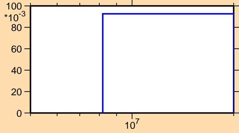
\sigma vs. E for ^{90}\text{Rb}(n,3n)
