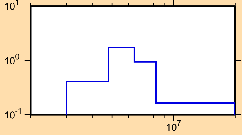
\sigma vs. E for ^{90}\text{Rb}(n,n\text{cont.})
