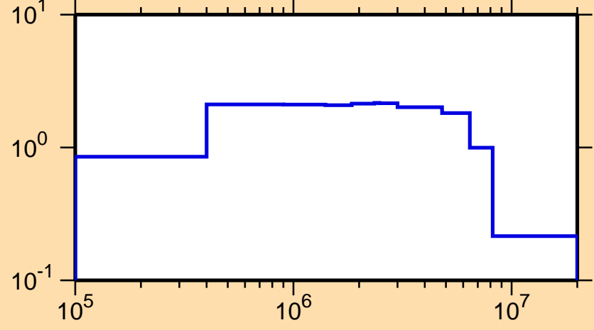
\sigma vs. E for ^{90}\text{Rb}(n,\text{inel.})
