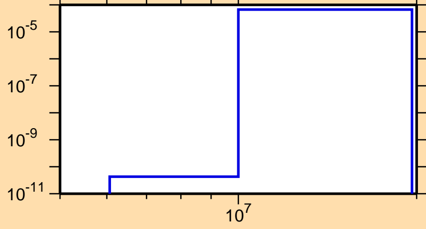
\sigma vs. E for ^{90}\text{Rb}(n,t)
