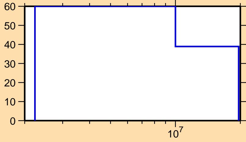
\Delta\sigma/\sigma vs. E for ^{90}\text{Rb}(n,\gamma)
