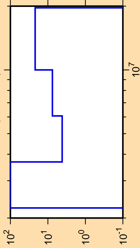
\Delta\sigma/\sigma vs. E for ^{90}\text{Rb}(n,\text{ncont.})
