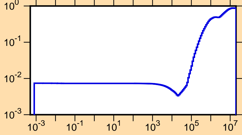
\mu vs. E for ^{91}\text{Rb}(\text{mt251})
