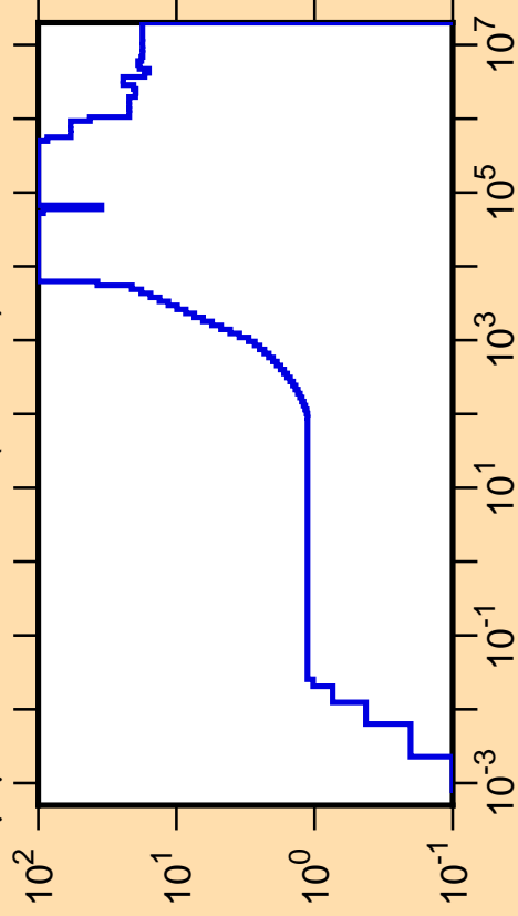
\Delta\mu/\mu vs. E for ^{91}\text{Rb}(\text{mt251})
