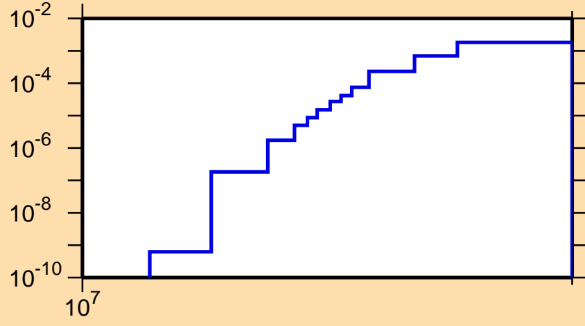
\sigma vs. E for ^{91}\text{Rb}(n,np)
