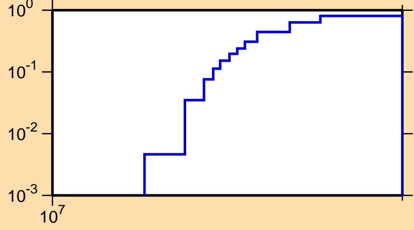
\sigma vs. E for ^{91}\text{Rb}(n,3n)
