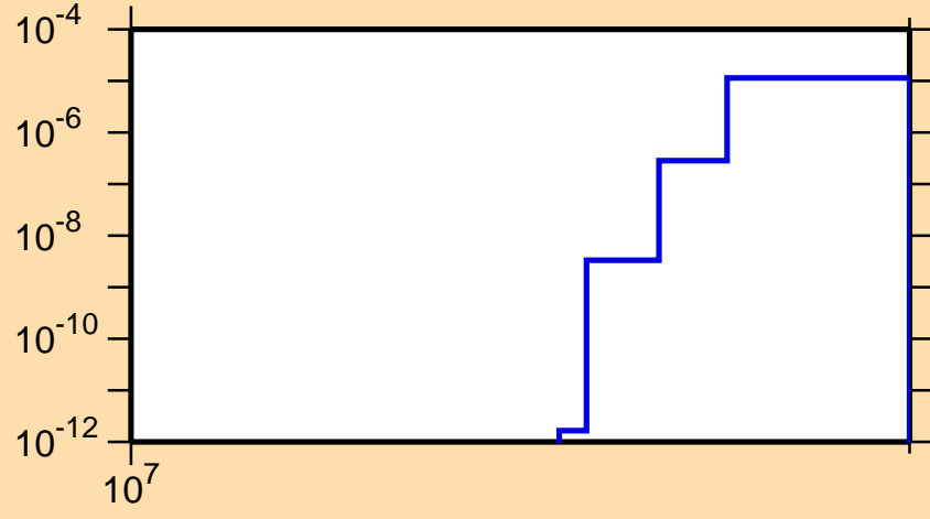
\sigma vs. E for ^{91}\text{Rb}(n,nt)
