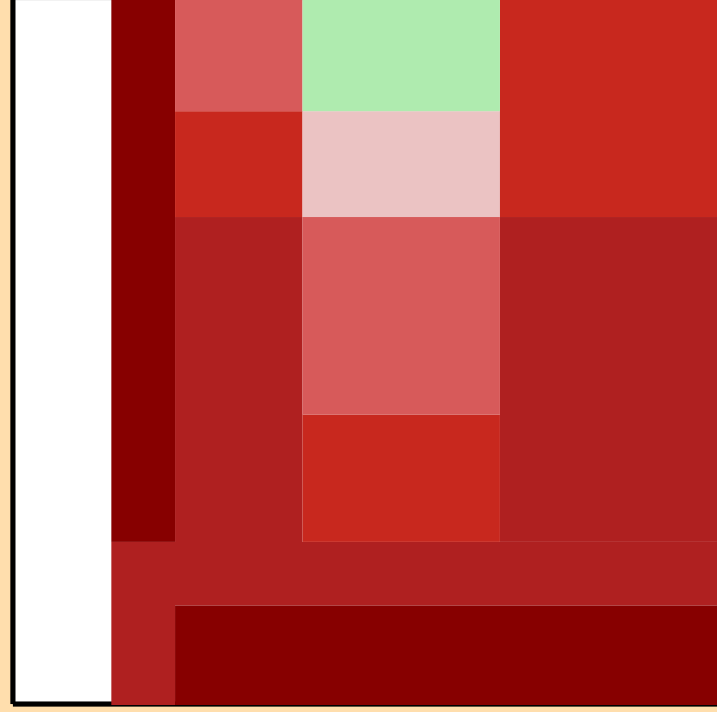
\Delta\sigma/\sigma vs. E for ^{91}\text{Rb}(n,p)
