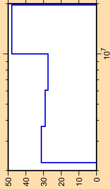
\Delta\sigma/\sigma vs. E for ^{91}\text{Rb}(n,\text{ncont.})
