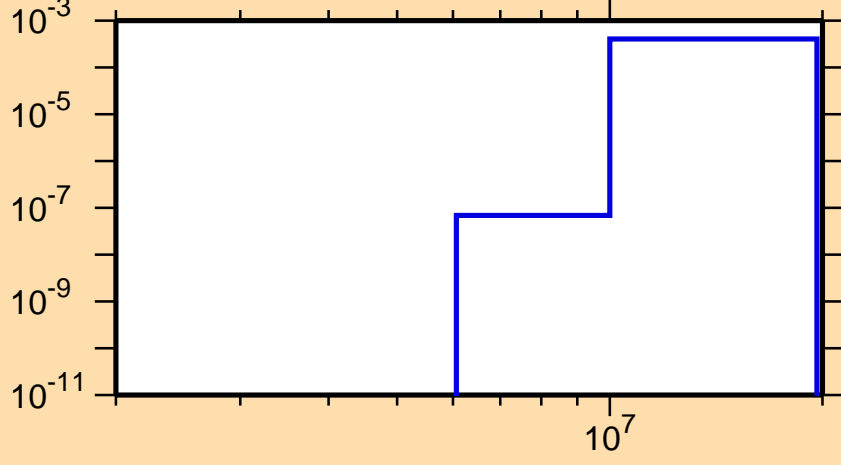
\sigma vs. E for ^{91}\text{Rb}(n,\alpha)
