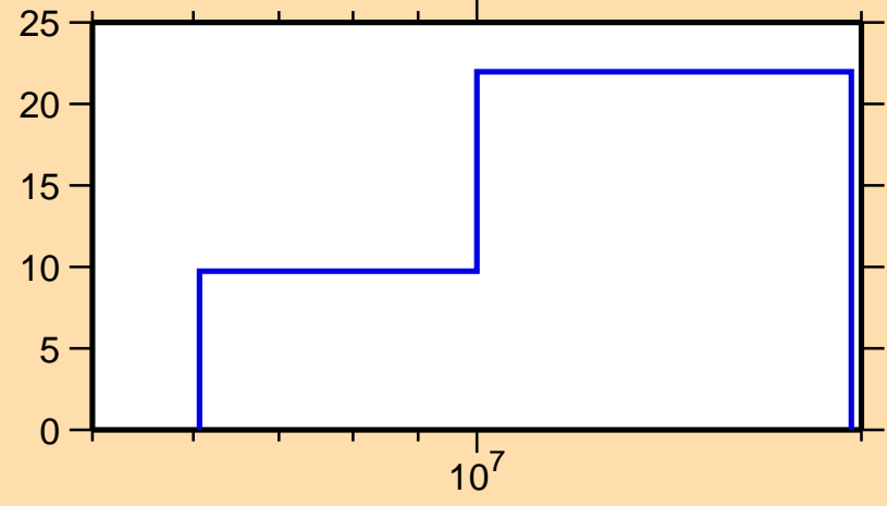
\Delta\sigma/\sigma vs. E for ^{91}\text{Rb}(n,el.)
