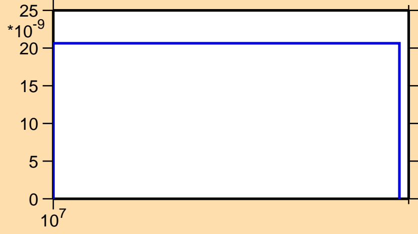
\sigma vs. E for ^{91}\text{Rb}(n,nd)
