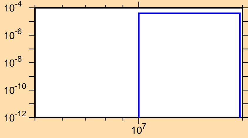
\sigma vs. E for ^{91}\text{Rb}(n,t)
