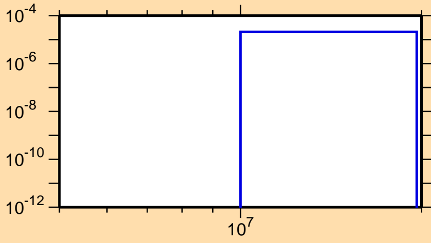
\sigma vs. E for ^{91}\text{Rb}(n,\alpha)
