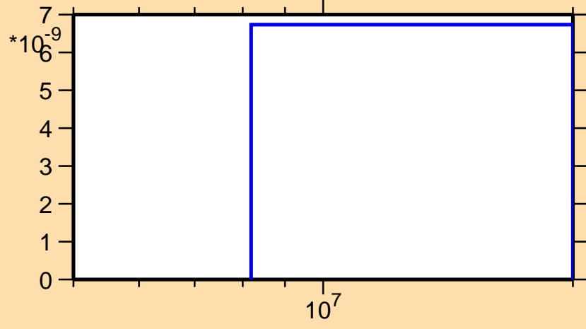
\sigma vs. E for ^{93}\text{Rb}(n,nd)
