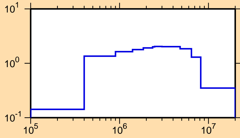
\sigma vs. E for ^{93}\text{Rb}(n,\text{inel.})
