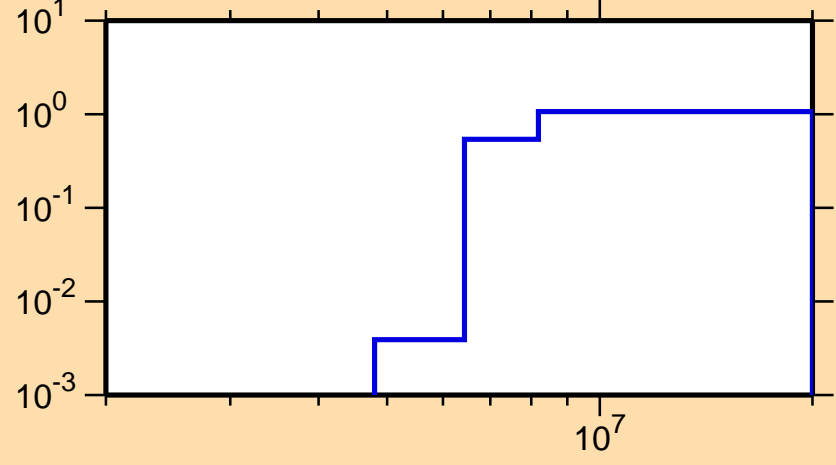
\sigma vs. E for ^{93}\text{Rb}(n,2n)
