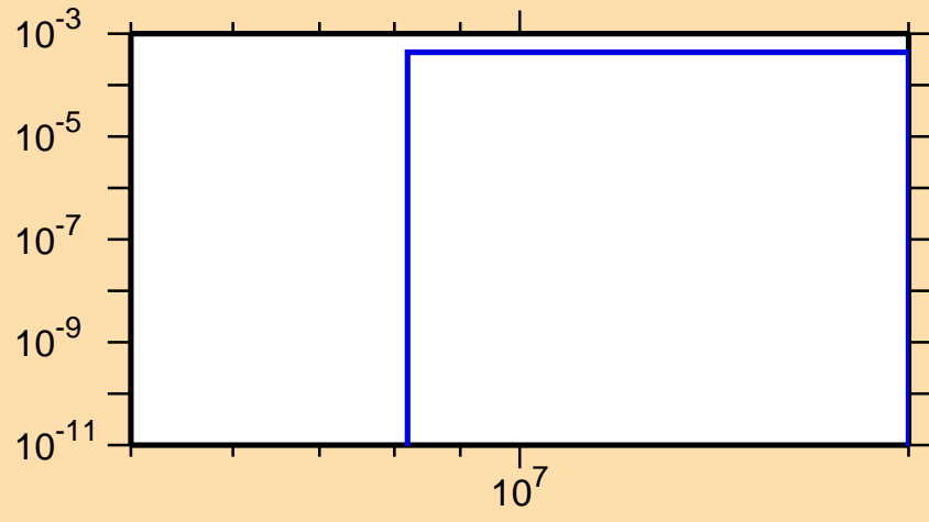
\sigma vs. E for ^{93}\text{Rb}(n,p)
