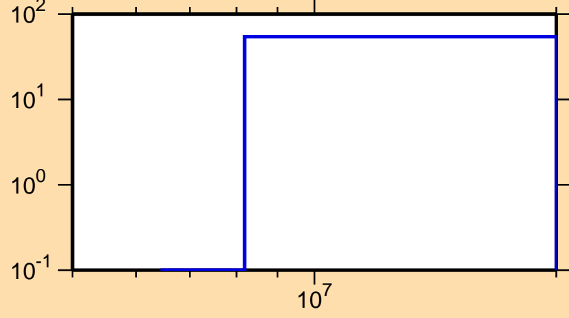
\Delta\sigma/\sigma vs. E for ^{93}\text{Rb}(n,p)
