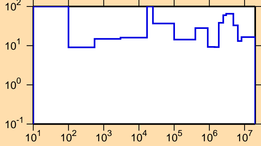
\Delta\sigma/\sigma vs. E for ^{94}\text{Rb}(n,\text{el.})
