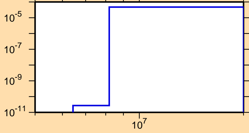
\sigma vs. E for ^{94}\text{Rb}(n,\alpha)
