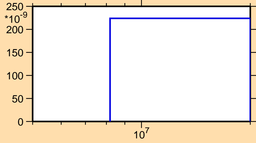
\sigma vs. E for ^{94}\text{Rb}(n,nd)
