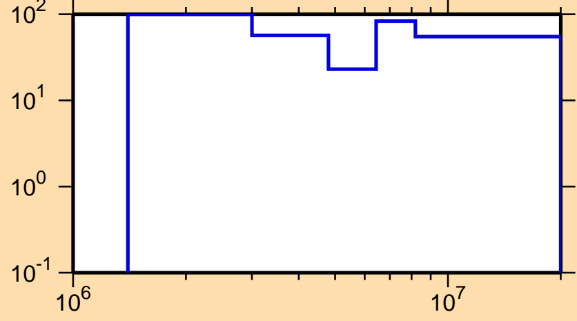
\Delta\sigma/\sigma vs. E for ^{94}\text{Rb}(n,n\text{cont.})
