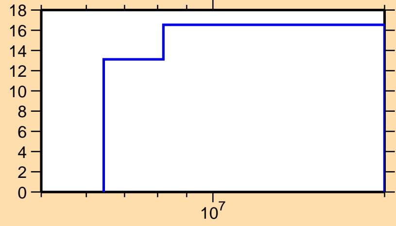
\Delta\sigma/\sigma vs. E for ^{94}\text{Rb}(n,el.)
