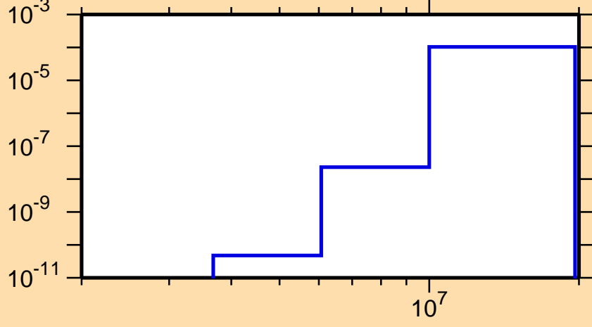
\sigma vs. E for ^{165}\text{Re}(n,\text{He3})
