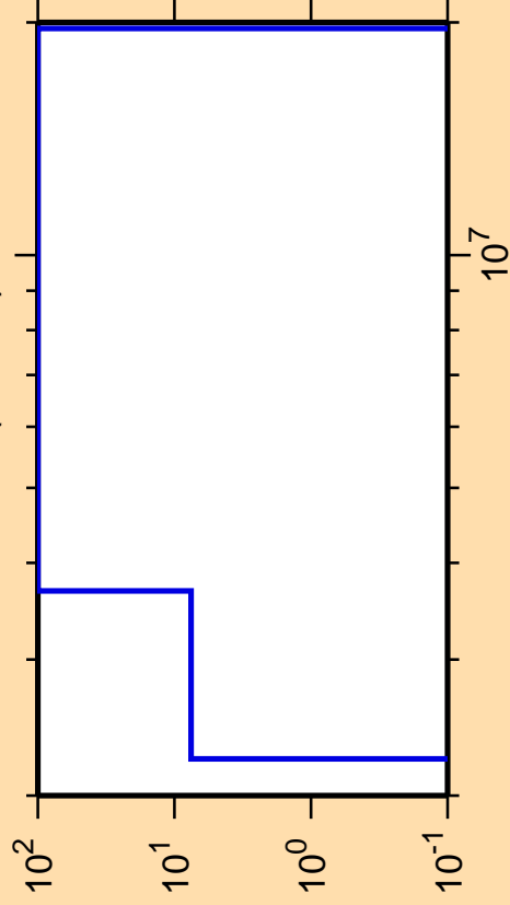
\Delta\sigma/\sigma vs. E for ^{165}\text{Re}(n,\text{He3})
