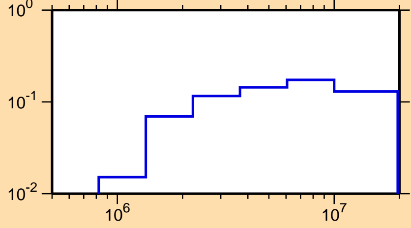
\sigma vs. E for ^{165}\text{Re}(n,n\text{cont.})
