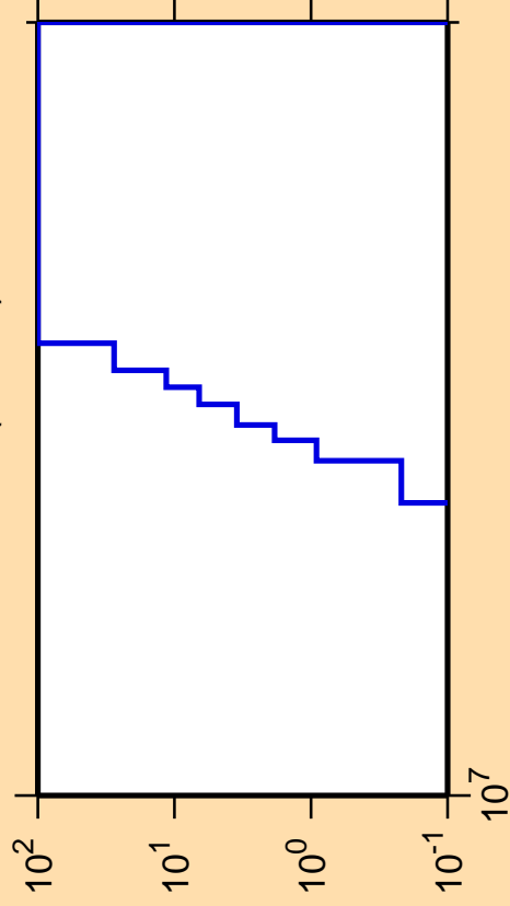
\Delta\sigma/\sigma vs. E for ^{165}\text{Re}(mt\ 34)
