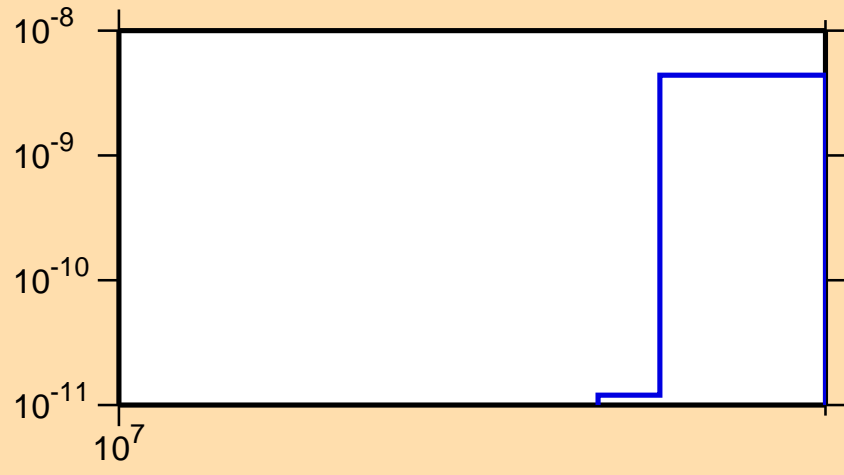
\sigma vs. E for ^{165}\text{Re}(n,nt)
