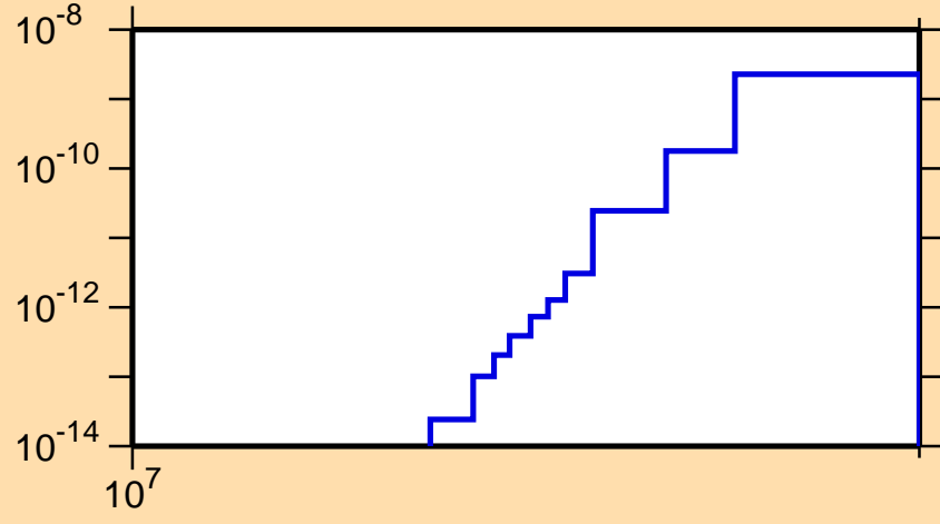
\sigma vs. E for ^{165}\text{Re}(mt\ 34)
