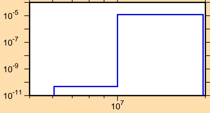
\sigma vs. E for ^{165}\text{Re}(n,\text{pd})
