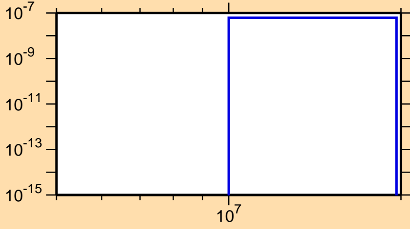
\sigma vs. E for ^{165}\text{Re}(n,\text{nd})
