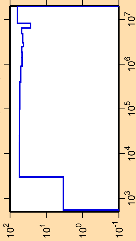
\Delta\sigma/\sigma vs. E for ^{165}\text{Re}(n,\text{inel.})
