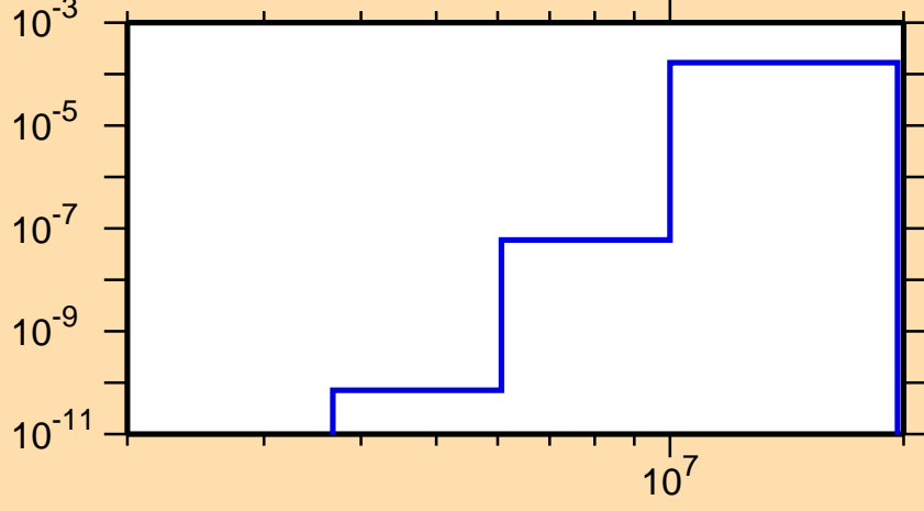
\sigma vs. E for ^{166}\text{Re}(n,\text{He3})
