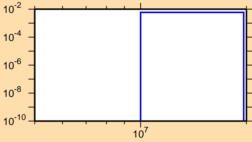
\sigma vs. E for ^{166}\text{Re}(n,2np)
