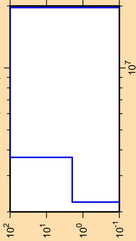
\Delta\sigma/\sigma vs. E for ^{166}\text{Re}(n,\text{He3})
