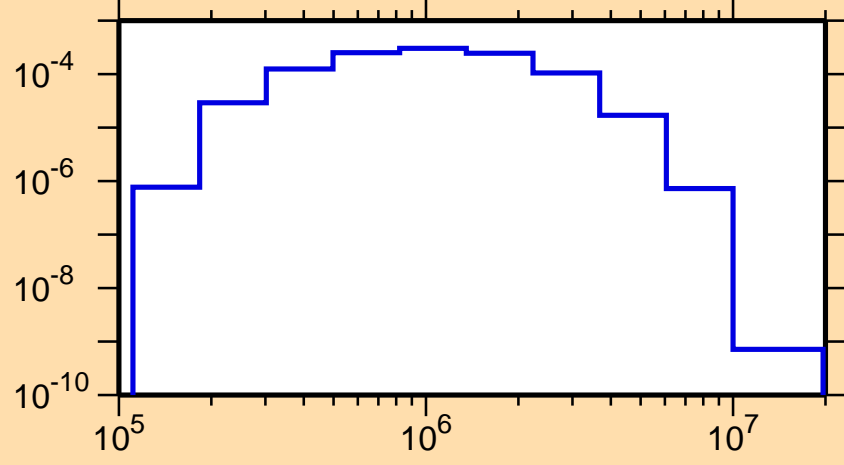
\sigma vs. E for ^{166}\text{Re}(n,n_1)
