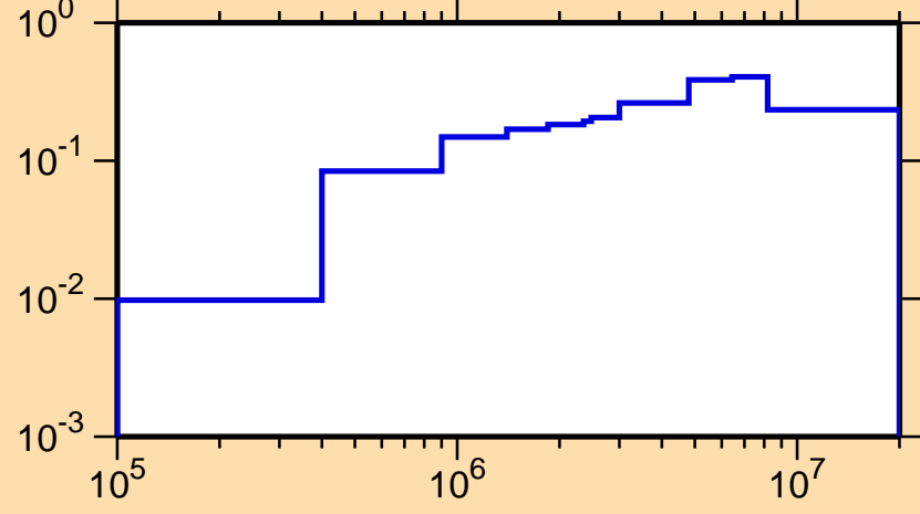
\sigma vs. E for ^{166}\text{Re}(n,\text{inel.})
