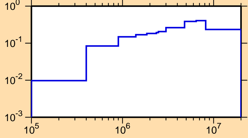
\sigma vs. E for ^{166}\text{Re}(n,n\text{cont.})
