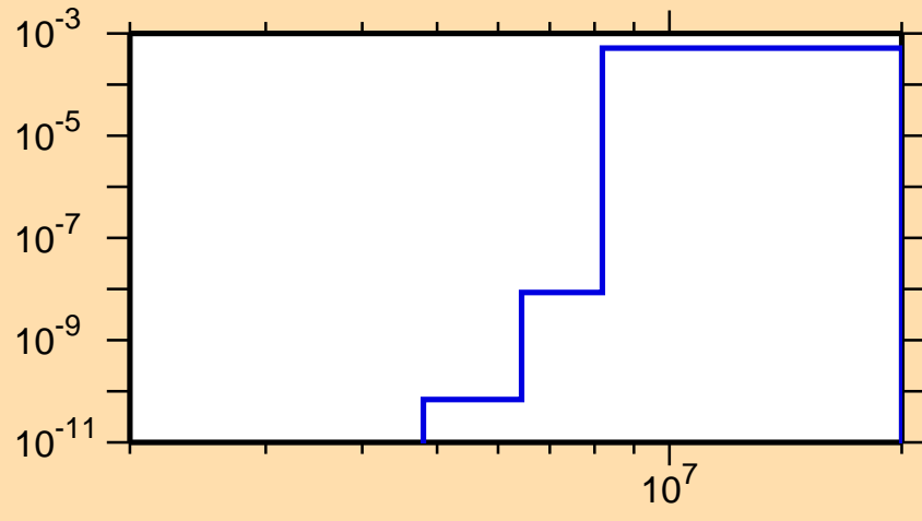
\sigma vs. E for ^{166}\text{Re}(\text{mt } 45)
