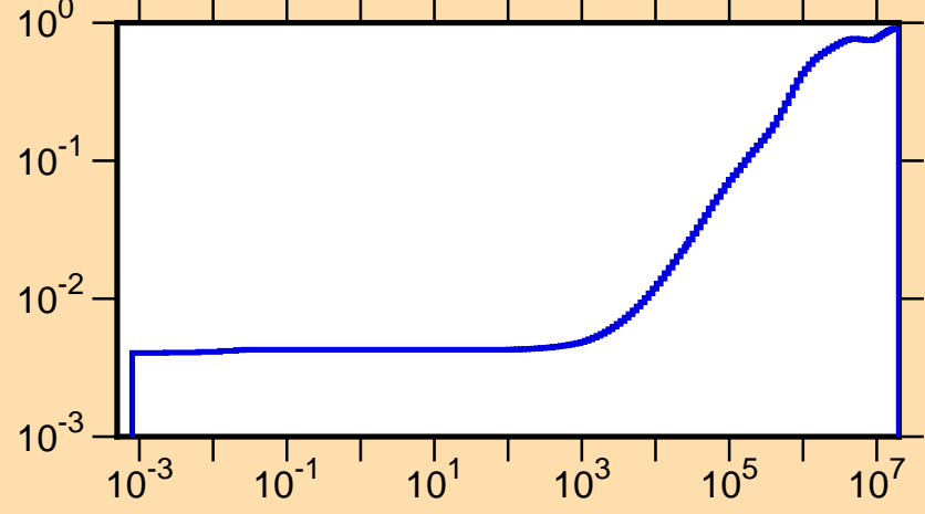
\mu vs. E for ^{167}\text{Re}(\text{mt251})
