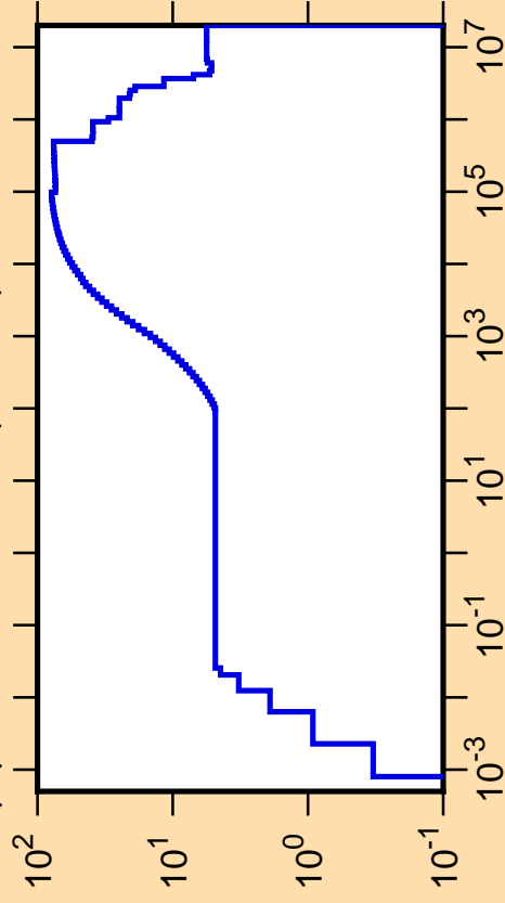
\Delta\mu/\mu vs. E for ^{167}\text{Re}(\text{mt251})
