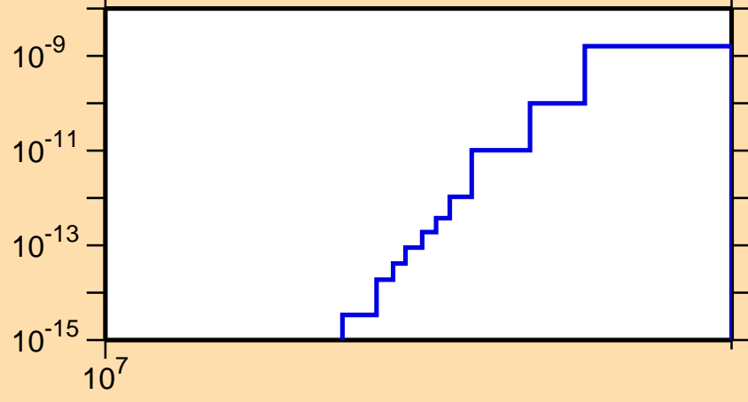
\sigma vs. E for ^{167}\text{Re}(mt\ 34)
