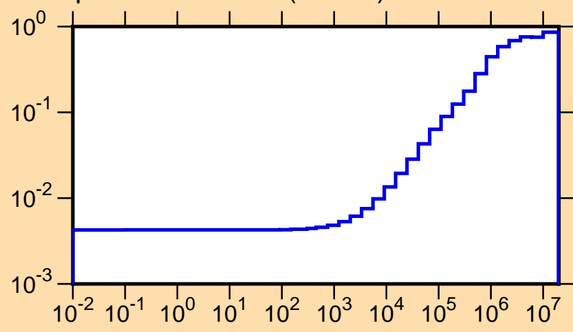
\mu vs. E for ^{167}\text{Re}(\text{mt251})
