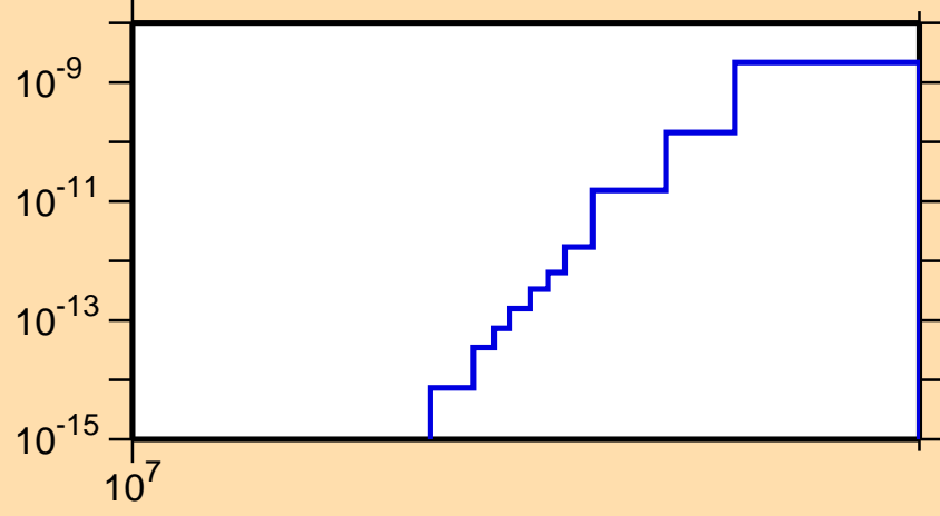
\sigma vs. E for ^{167}\text{Re}(mt\ 34)
