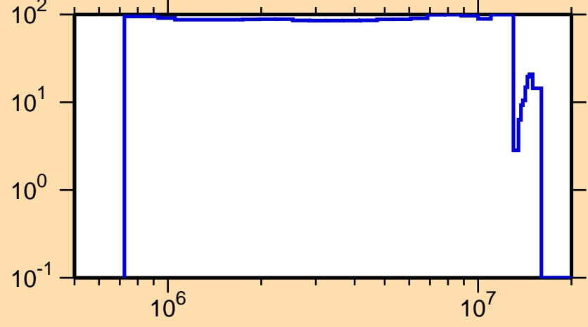
\Delta\sigma/\sigma vs. E for ^{167}\text{Re}(n,n_1)
