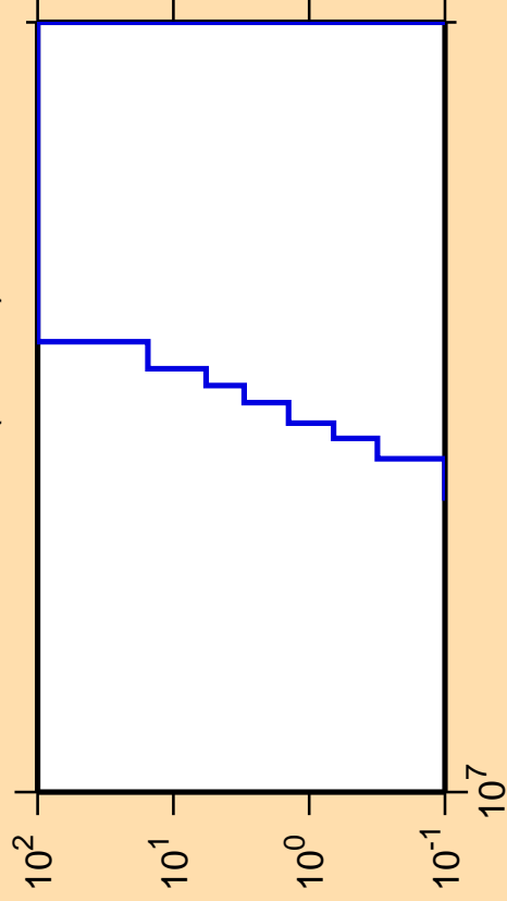
\Delta\sigma/\sigma vs. E for ^{167}\text{Re}(mt\ 34)
