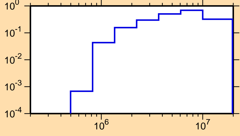
\sigma vs. E for ^{167}\text{Re}(n,n\text{cont.})
