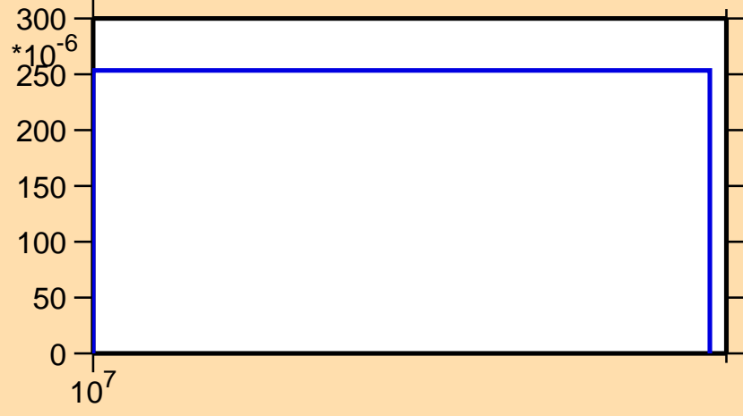
\sigma vs. E for ^{167}\text{Re}(n,2np)
