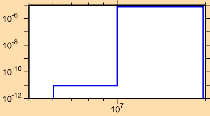
\sigma vs. E for ^{167}\text{Re}(n,\text{pd})
