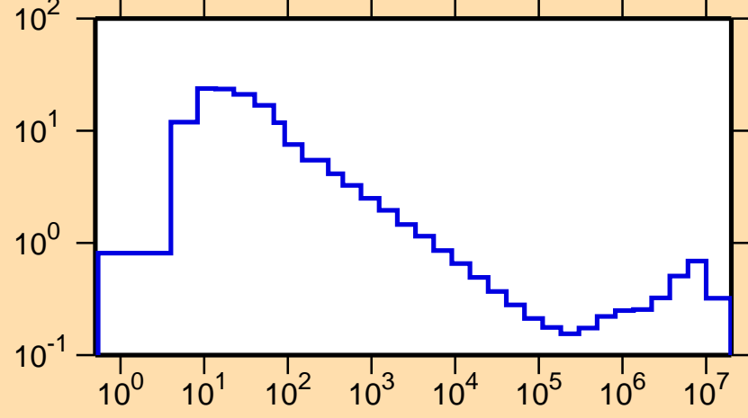
\sigma vs. E for ^{167}\text{Re}(n,\text{inel.})
