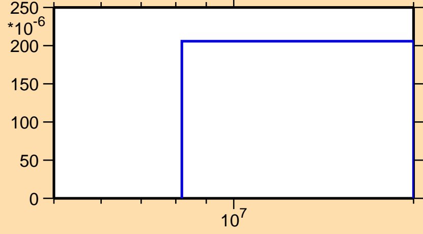
\sigma vs. E for ^{167}\text{Re}(n,2np)
