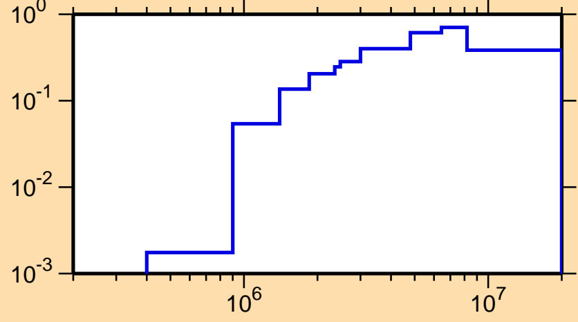
\sigma vs. E for ^{167}\text{Re}(n,n\text{cont.})
