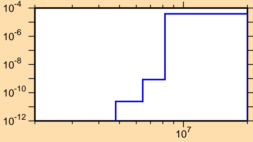
\sigma vs. E for ^{167}\text{Re}(n,\text{He3})
