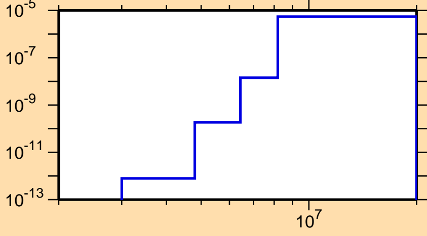
\sigma vs. E for ^{167}\text{Re}(mt117)
