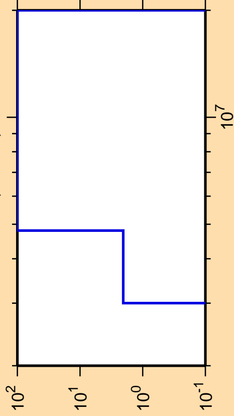
\Delta\sigma/\sigma vs. E for ^{167}\text{Re}(n,\text{He3})
