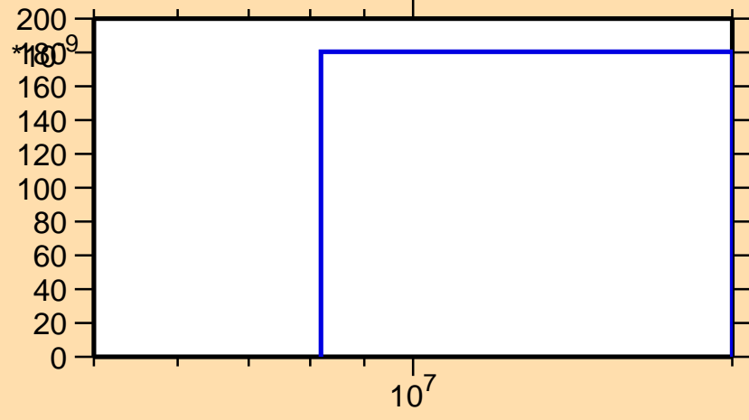
\sigma vs. E for ^{167}\text{Re}(n,\text{nd})
