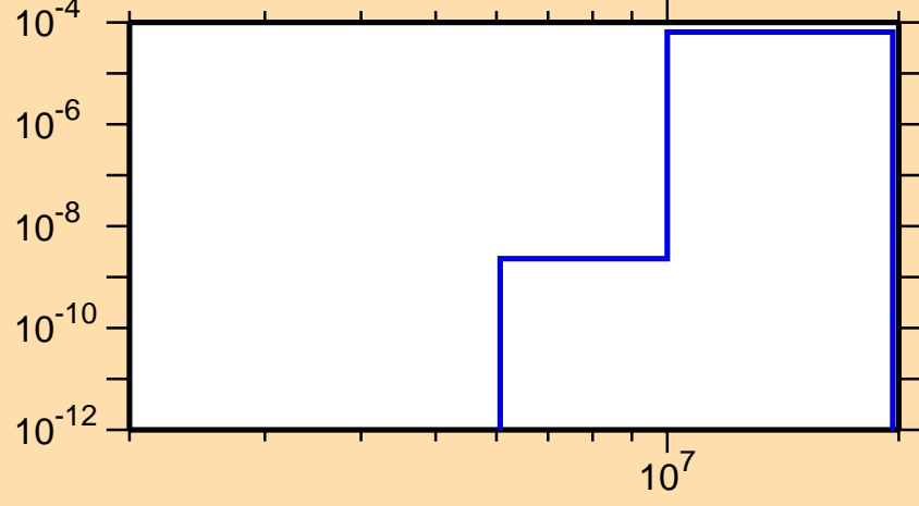
\sigma vs. E for ^{169}\text{Re}(\text{mt } 45)
