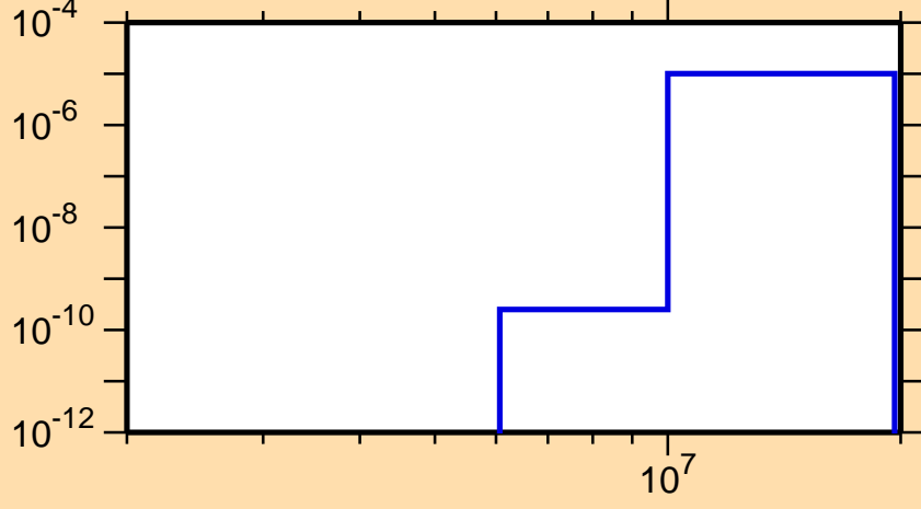
\sigma vs. E for ^{169}\text{Re}(n,\text{He3})
