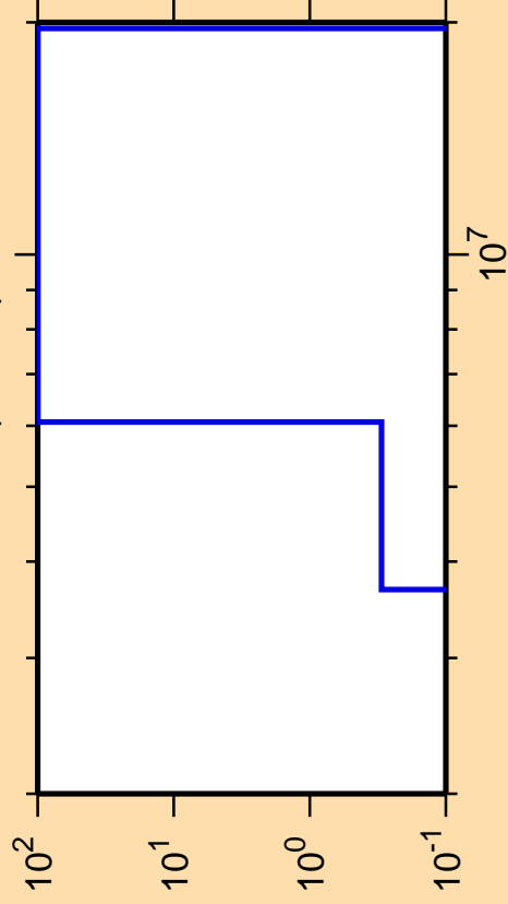
\Delta\sigma/\sigma vs. E for ^{169}\text{Re}(\text{mt } 45)
