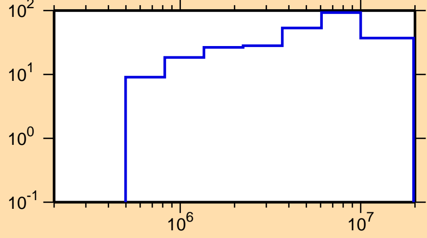
\Delta\sigma/\sigma vs. E for ^{169}\text{Re}(n,\text{el.})
