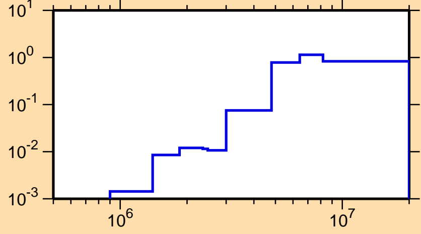
\sigma vs. E for ^{169}\text{Re}(n,n\text{cont.})
