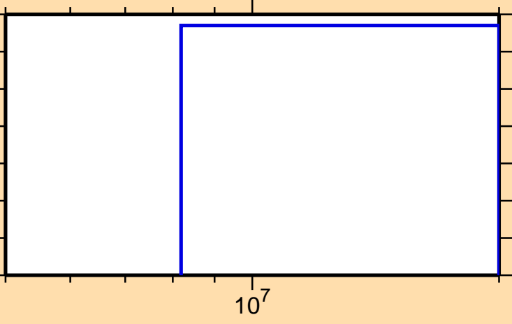
\sigma vs. E for ^{169}\text{Re}(n,\text{pd})
