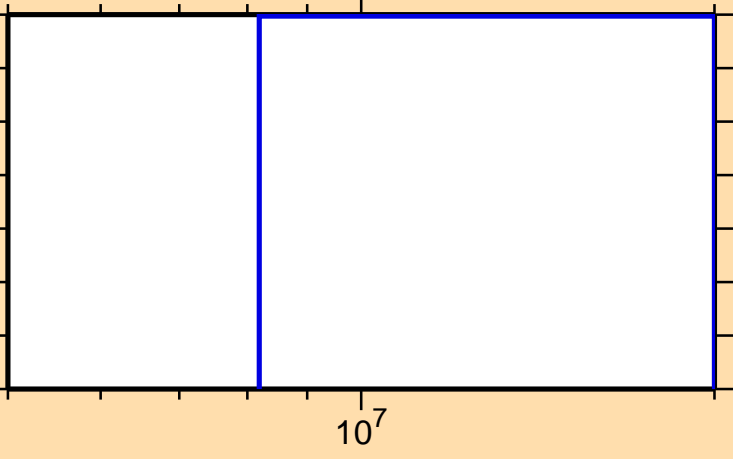
\sigma vs. E for ^{169}\text{Re}(n,2np)
