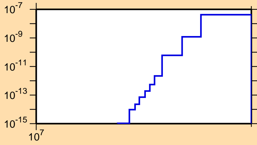
\sigma vs. E for ^{169}\text{Re}(n,\text{pt})
