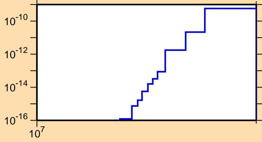
\sigma vs. E for ^{169}\text{Re}(mt\ 34)
