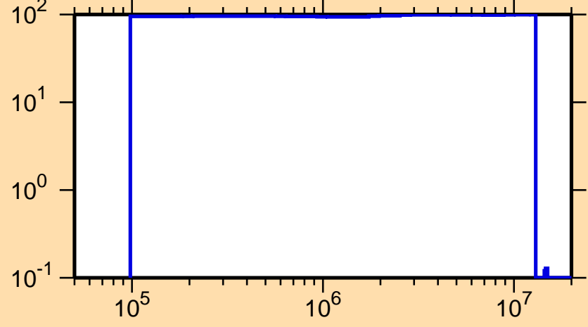
\Delta\sigma/\sigma vs. E for ^{169}\text{Re}(n,n_1)
