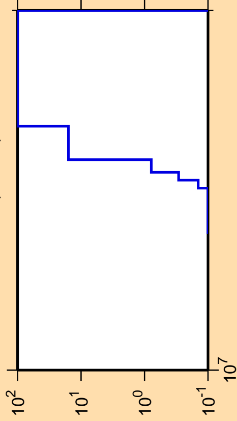
\Delta\sigma/\sigma vs. E for ^{169}\text{Re}(mt\ 34)
