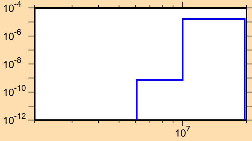
\sigma vs. E for ^{169}\text{Re}(n,\text{He3})
