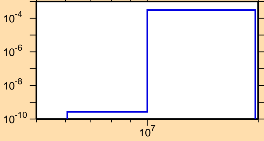
\sigma vs. E for ^{169}\text{Re}(n,t)
