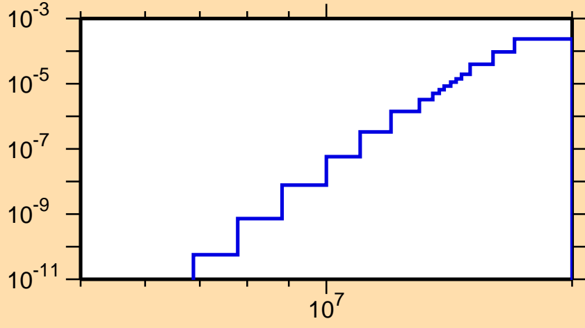
\sigma vs. E for ^{170}\text{Re}(n,\text{He}3)
