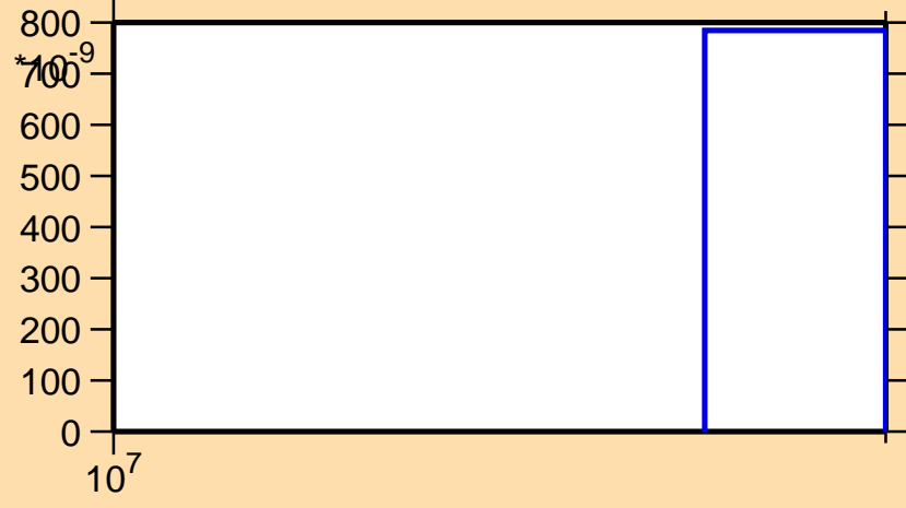
\sigma vs. E for ^{170}\text{Re}(n,3n)
