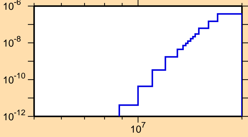
\sigma vs. E for ^{170}\text{Re}(\text{mt117})
