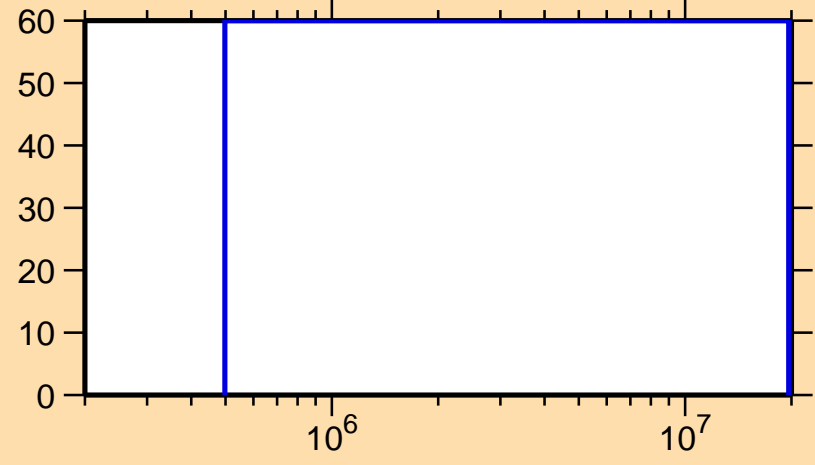
\Delta\sigma/\sigma vs. E for ^{170}\text{Re}(n,n_1)
