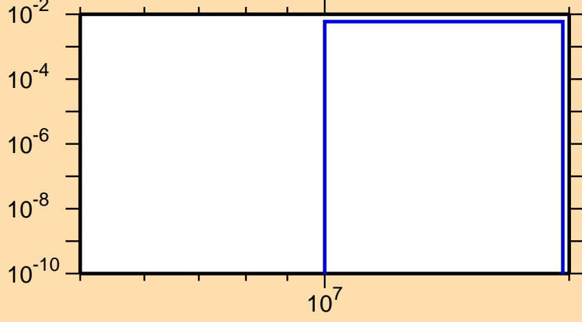
\sigma vs. E for ^{170}\text{Re}(n,2np)
