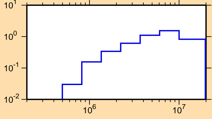
\sigma vs. E for ^{170}\text{Re}(n,n\text{cont.})
