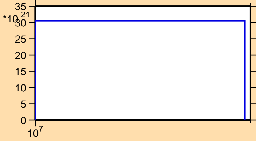
\sigma vs. E for ^{170}\text{Re}(\text{mt 11})
