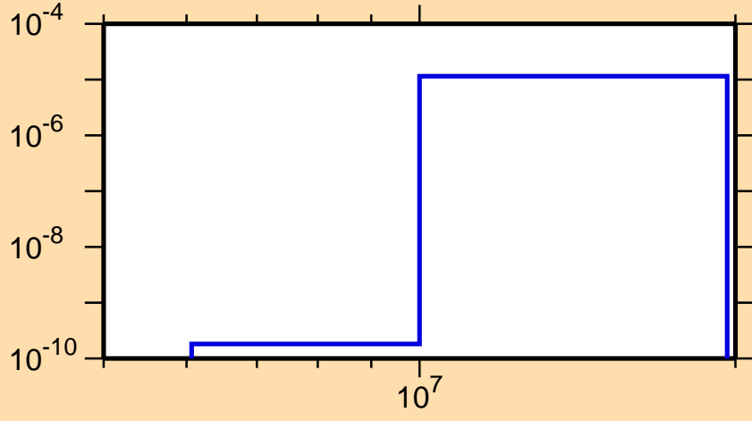
\sigma vs. E for ^{170}\text{Re}(\text{mt } 45)
