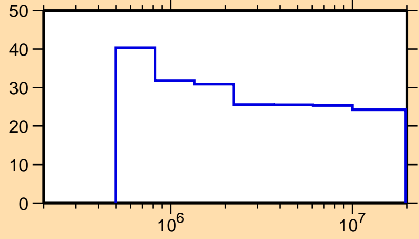
\Delta\sigma/\sigma vs. E for ^{170}\text{Re}(n,\text{nonel.})
