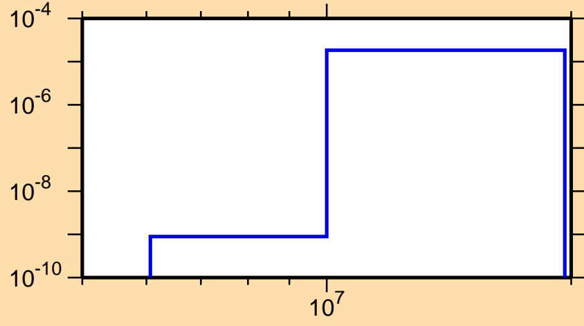
\sigma vs. E for ^{170}\text{Re}(n,\text{He3})
