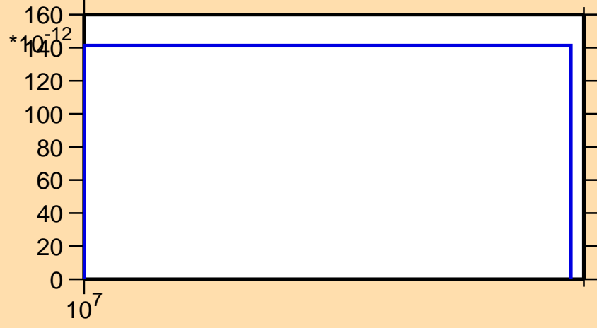
\sigma vs. E for ^{170}\text{Re}(\text{mt } 34)
