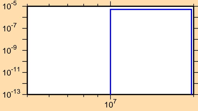
\sigma vs. E for ^{170}\text{Re}(n,\text{nd})
