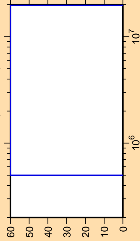
\Delta\sigma/\sigma vs. E for ^{170}\text{Re}(n,n\text{cont.})
