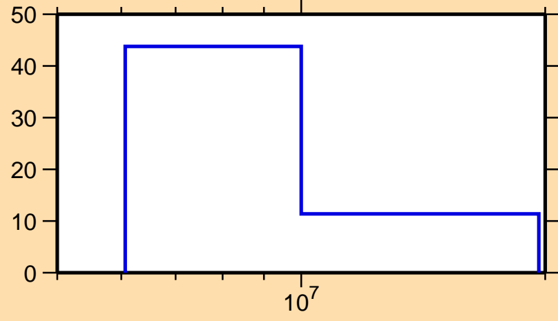
\Delta\sigma/\sigma vs. E for ^{170}\text{Re}(n,\text{el.})
