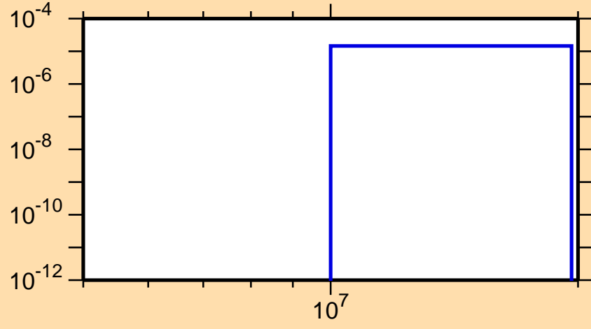
\sigma vs. E for ^{170}\text{Re}(n,2n\alpha)
