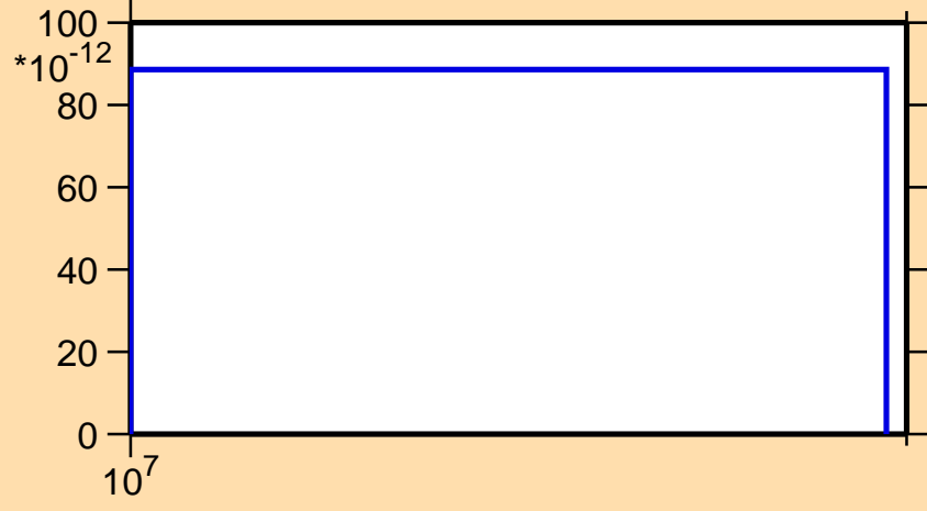
\sigma vs. E for ^{170}\text{Re}(n,nt)
