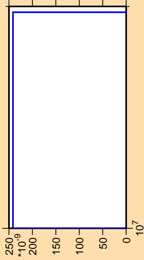
\Delta\sigma/\sigma vs. E for ^{170}\text{Re}(\text{mt 11})
