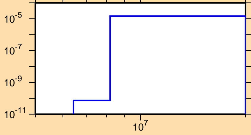
\sigma vs. E for ^{170}\text{Re}(n,\text{He3})
