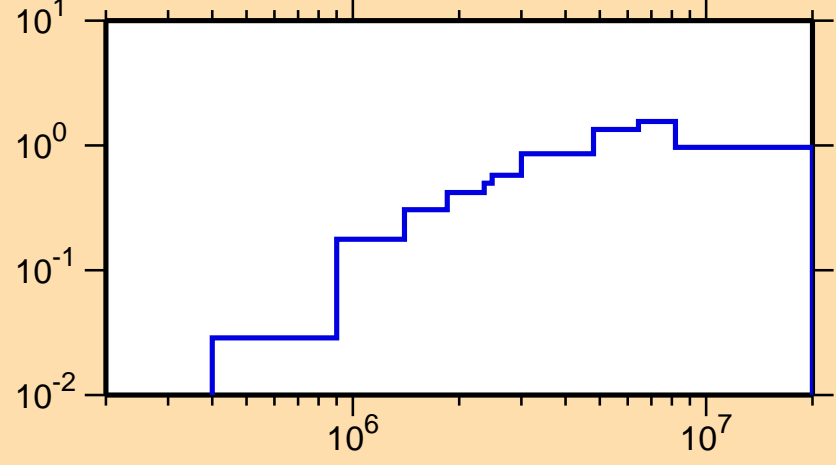
\sigma vs. E for ^{170}\text{Re}(n,n\text{cont.})
