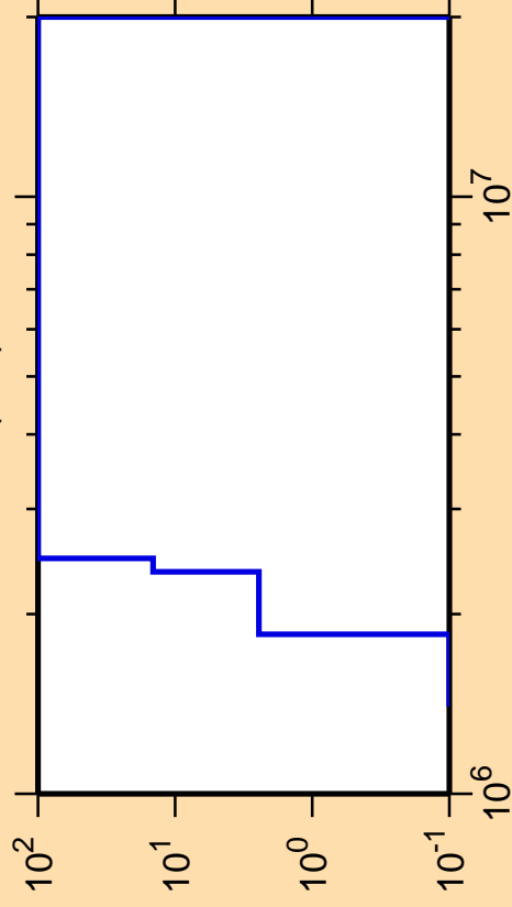
\Delta\sigma/\sigma vs. E for ^{170}\text{Re}(n,d)
