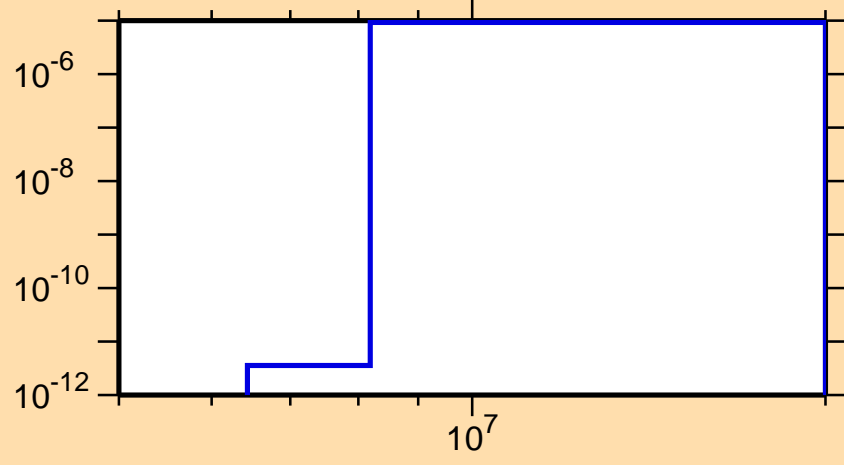
\sigma vs. E for ^{170}\text{Re}(\text{mt } 45)
