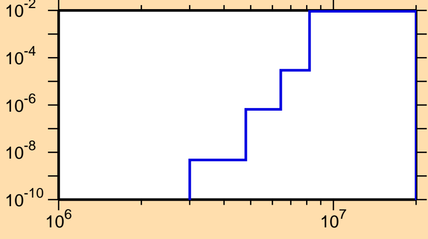
\sigma vs. E for ^{170}\text{Re}(n,d)
