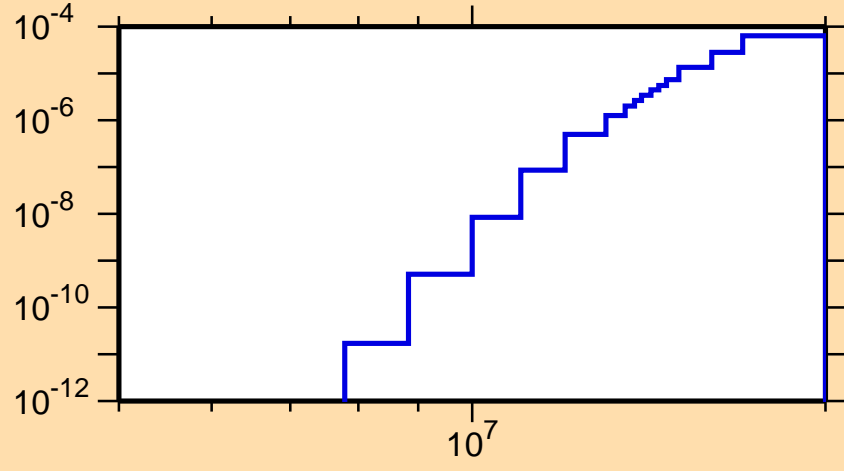
\sigma vs. E for ^{171}\text{Re}(\text{mt } 45)
