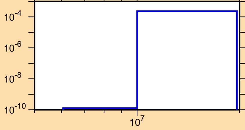
\sigma vs. E for ^{171}\text{Re}(n,t)
