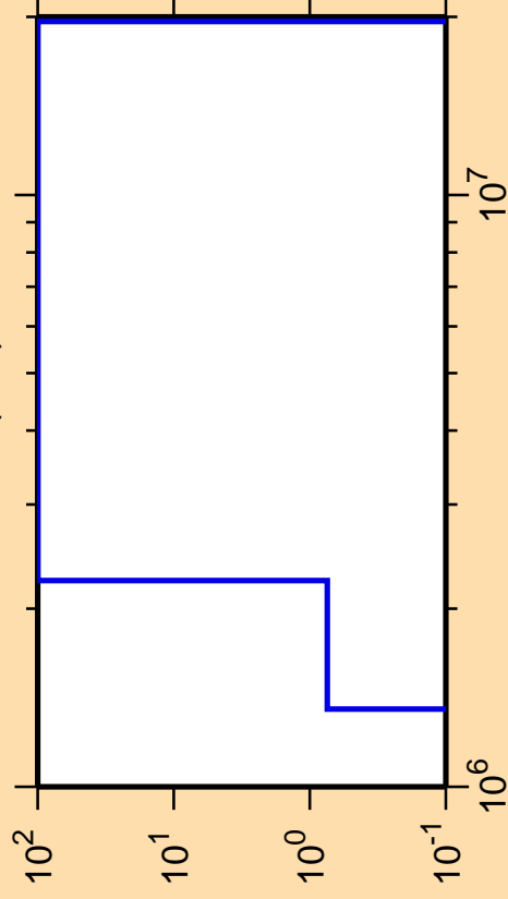
\Delta\sigma/\sigma vs. E for ^{171}\text{Re}(n,d)
