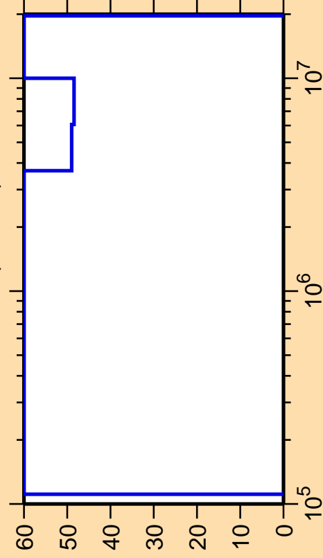
\Delta\sigma/\sigma vs. E for ^{171}\text{Re}(n,\text{inel.})
