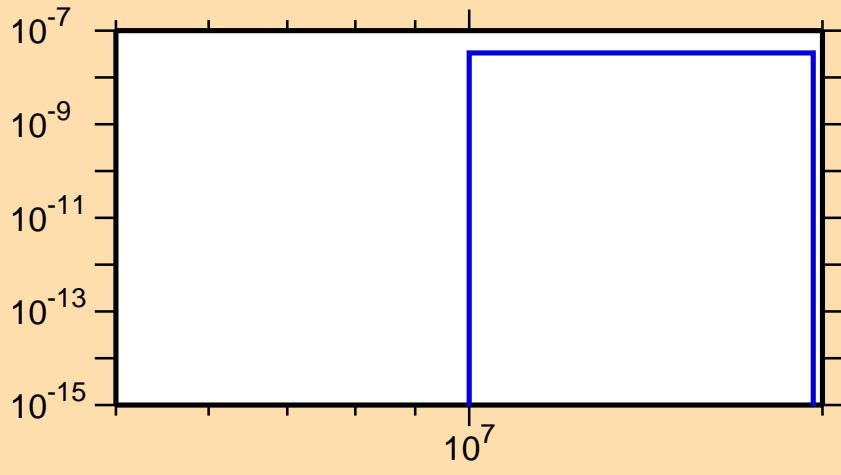
\sigma vs. E for ^{171}\text{Re}(n,\text{pd})
