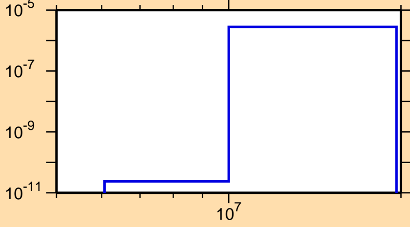
\sigma vs. E for ^{171}\text{Re}(n,\text{He3})
