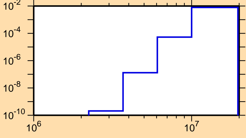
\sigma vs. E for ^{171}\text{Re}(n,d)
