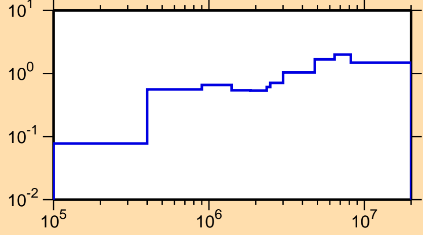
\sigma vs. E for ^{171}\text{Re}(n,\text{inel.})
