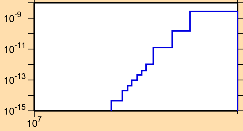
\sigma vs. E for ^{172}\text{Re}(\text{mt } 34)
