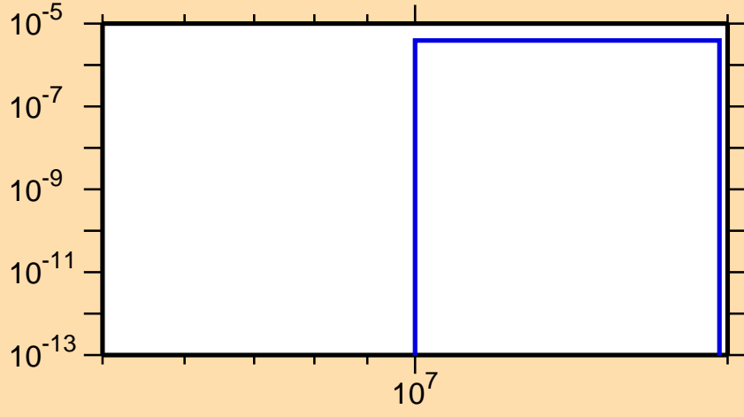
\sigma vs. E for ^{172}\text{Re}(n,\text{nd})
