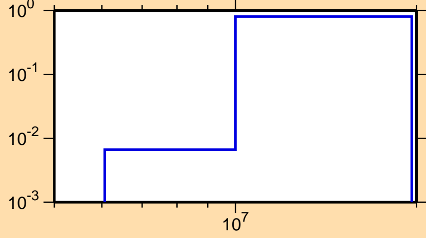
\sigma vs. E for ^{172}\text{Re}(n,2n)
