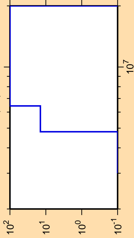
\Delta\sigma/\sigma vs. E for ^{172}\text{Re}(n,t)
