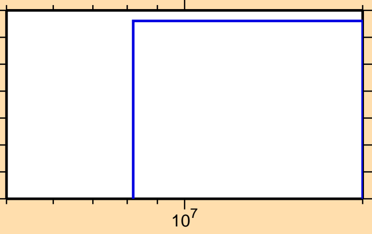
\sigma vs. E for ^{172}\text{Re}(n,\text{pt})
