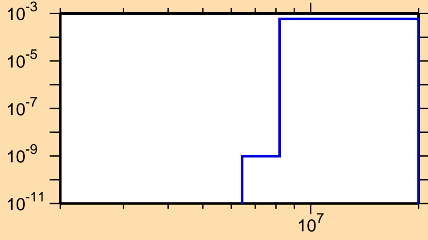
\sigma vs. E for ^{172}\text{Re}(n,t)
