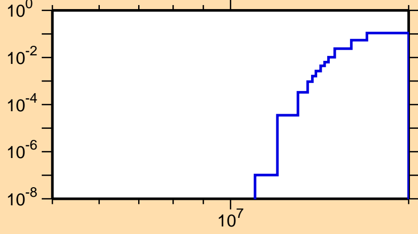
\sigma vs. E for ^{172}\text{Re}(n,2np)
