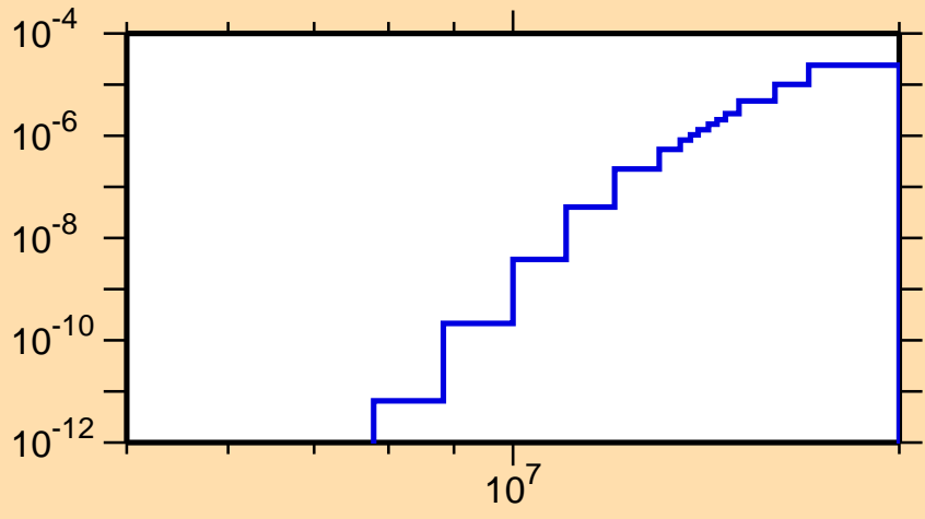
\sigma vs. E for ^{172}\text{Re}(\text{mt } 45)
