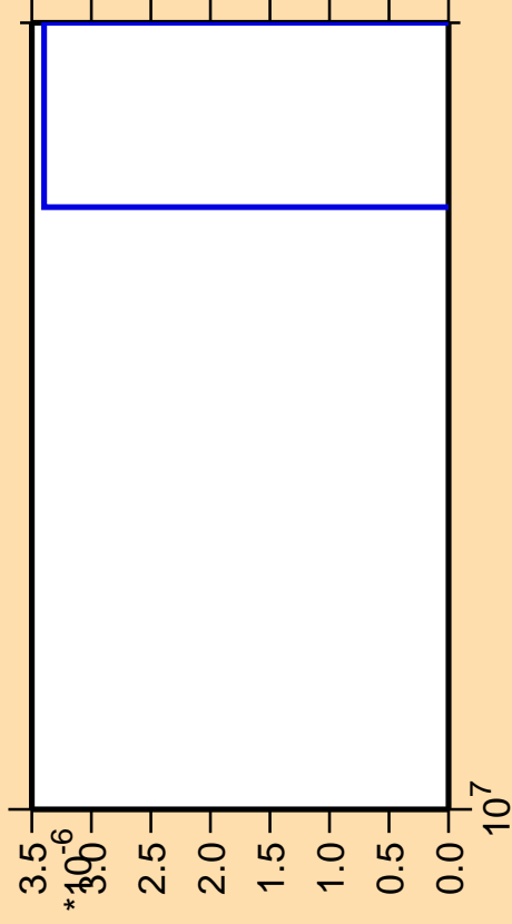
\Delta\sigma/\sigma vs. E for ^{172}\text{Re}(\text{mt } 42)
