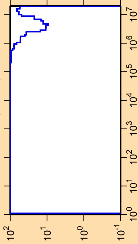
\Delta\sigma/\sigma vs. E for ^{172}\text{Re}(n,\text{inel.})
