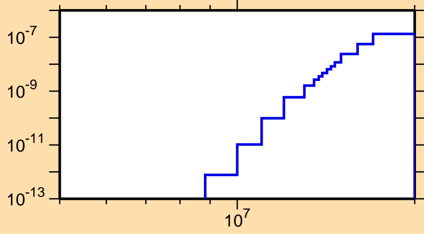
\sigma vs. E for ^{172}\text{Re}(\text{mt117})
