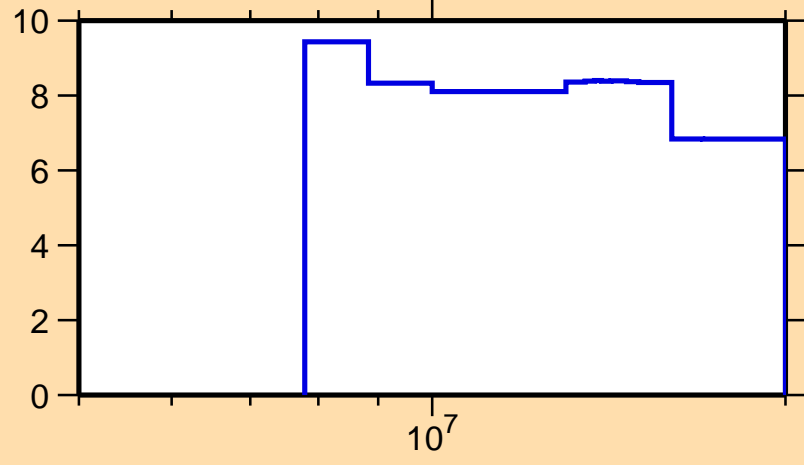
\Delta\sigma/\sigma vs. E for ^{172}\text{Re}(n,\text{nonel.})
