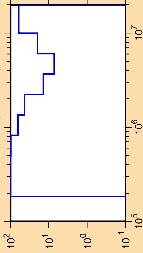
\Delta\sigma/\sigma vs. E for ^{172}\text{Re}(n,\text{ncont.})
