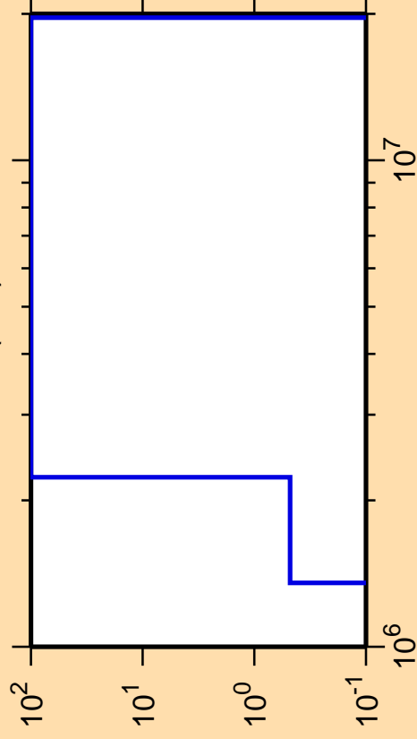
\Delta\sigma/\sigma vs. E for ^{172}\text{Re}(n,d)
