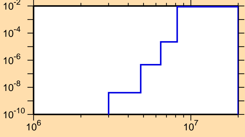
\sigma vs. E for ^{172}\text{Re}(n,d)
