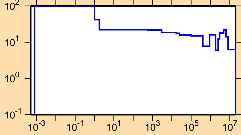
\Delta\sigma/\sigma vs. E for ^{172}\text{Re}(n,\text{el.})
