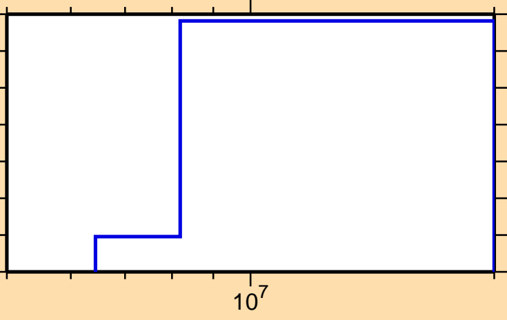
\sigma vs. E for ^{172}\text{Re}(n,\text{He3})
