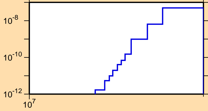
\sigma vs. E for ^{174}\text{Re}(n,\text{pd})
