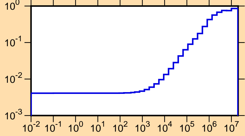
\mu vs. E for ^{174}\text{Re}(\text{mt251})
