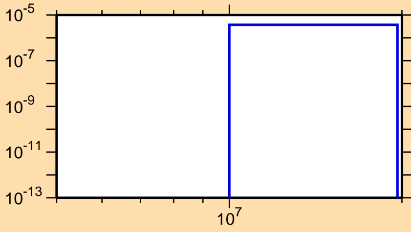
\sigma vs. E for ^{174}\text{Re}(n,\text{nd})
