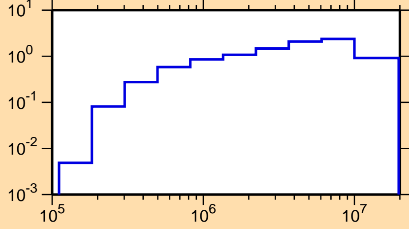
\sigma vs. E for ^{174}\text{Re}(n,\text{inel.})
