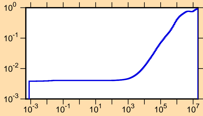
\mu vs. E for ^{176}\text{Re}(\text{mt251})
