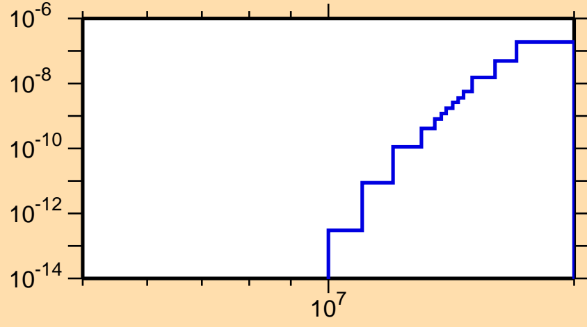
\sigma vs. E for ^{176}\text{Re}(\text{mt } 45)
