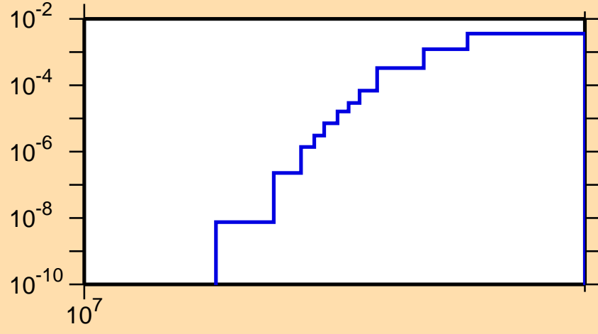
\sigma vs. E for ^{176}\text{Re}(n,2np)
