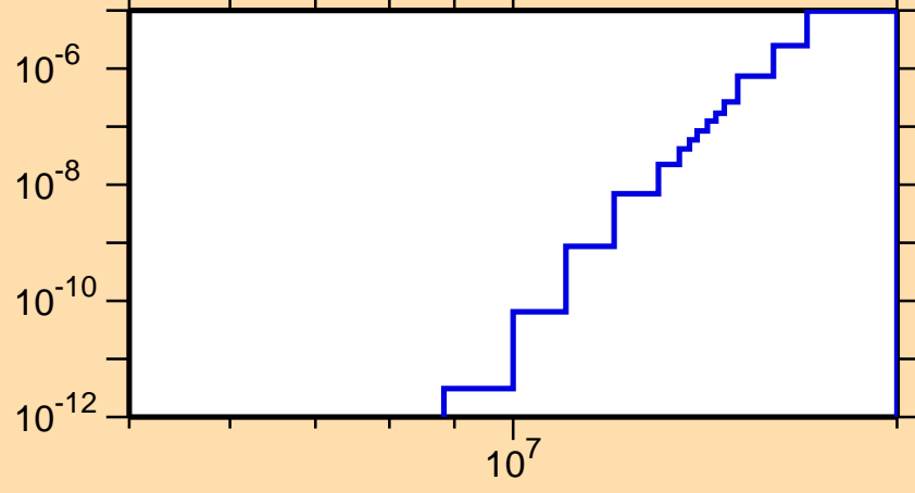
\sigma vs. E for ^{176}\text{Re}(n,\text{He3})
