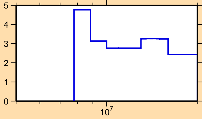
\Delta\sigma/\sigma vs. E for ^{176}\text{Re}(n,\text{nonel.})
