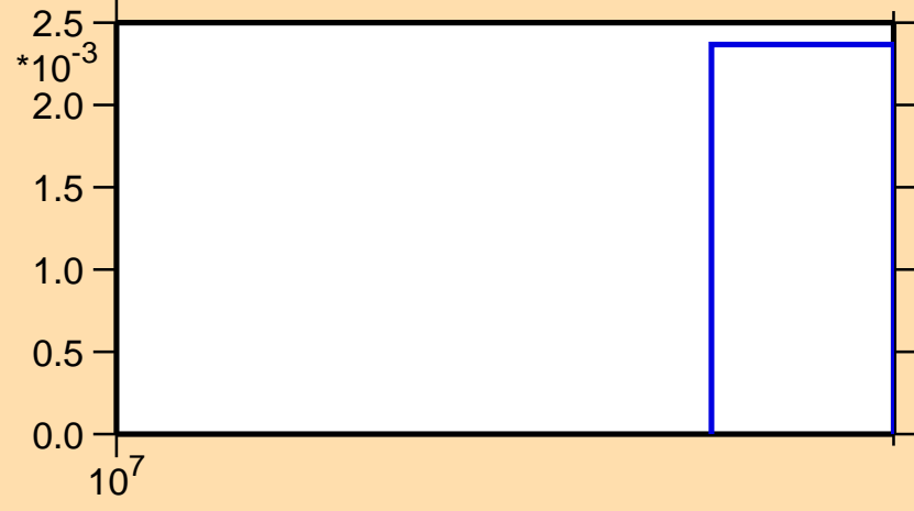
\sigma vs. E for ^{176}\text{Re}(n,3n)
