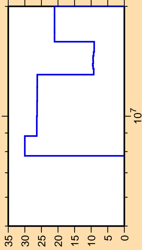
\Delta\sigma/\sigma vs. E for ^{176}\text{Re}(n,2n)
