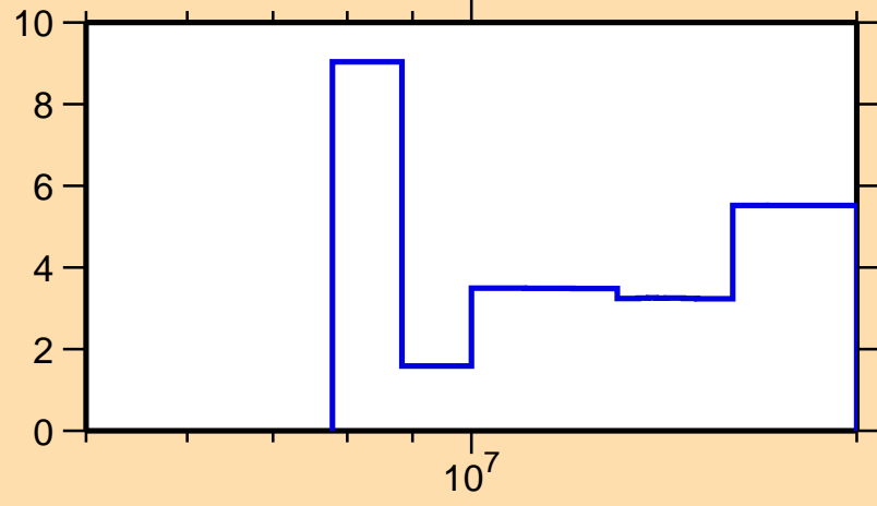
\Delta\sigma/\sigma vs. E for ^{176}\text{Re}(n,\text{el.})
