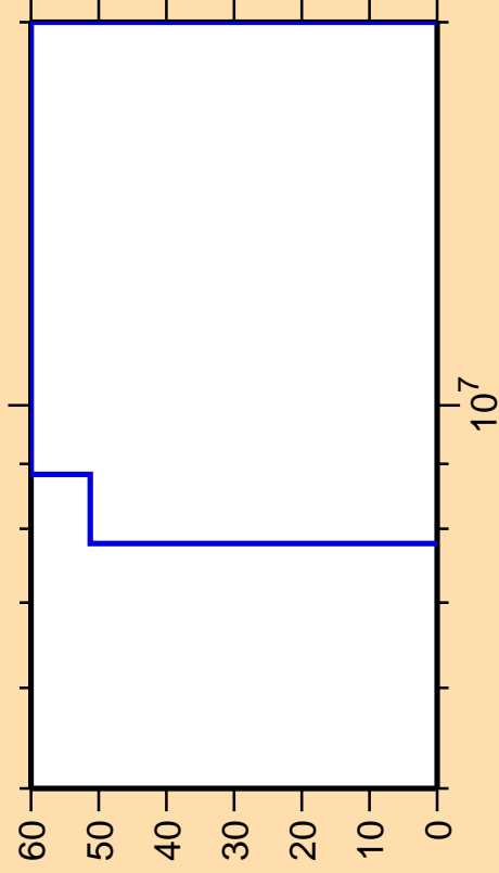
\Delta\sigma/\sigma vs. E for ^{176}\text{Re}(n,\gamma)
