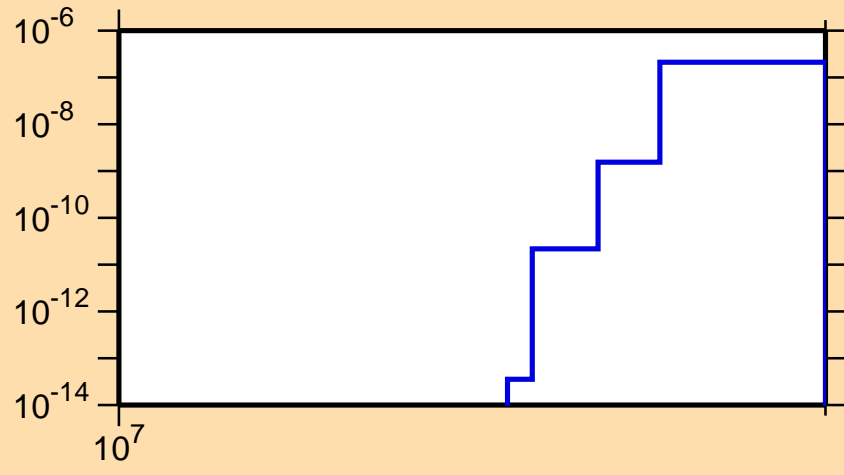
\sigma vs. E for ^{176}\text{Re}(n,nt)
