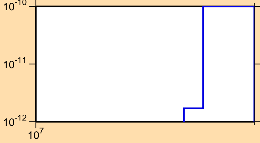
\sigma vs. E for ^{176}\text{Re}(\text{mt 34})
