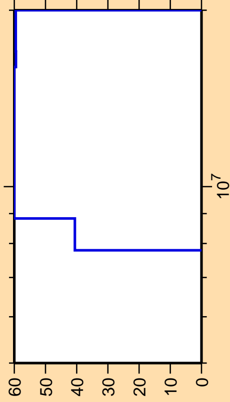
\Delta\sigma/\sigma vs. E for ^{176}\text{Re}(n,n\text{cont.})
