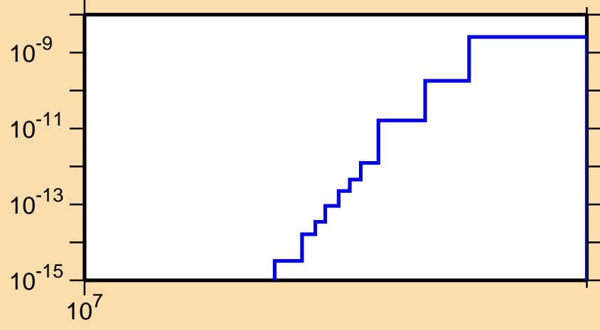
\sigma vs. E for ^{176}\text{Re}(n,\text{pd})
