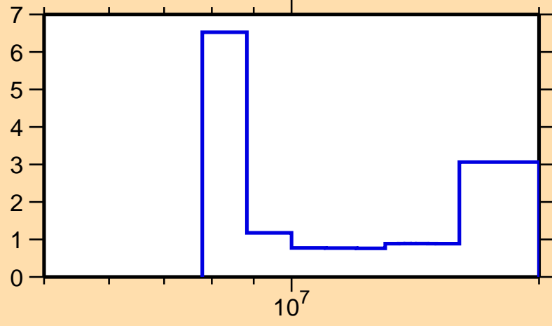
\Delta\sigma/\sigma vs. E for ^{176}\text{Re}(n,\text{tot.})
