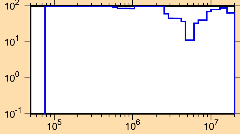
\Delta\sigma/\sigma vs. E for ^{176}\text{Re}(n,\text{inel.})
