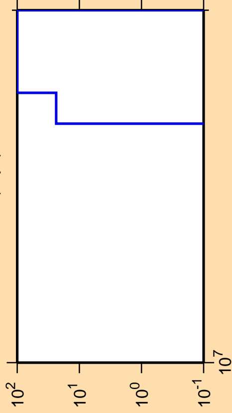
\Delta\sigma/\sigma vs. E for ^{176}\text{Re}(n,\text{pt})
