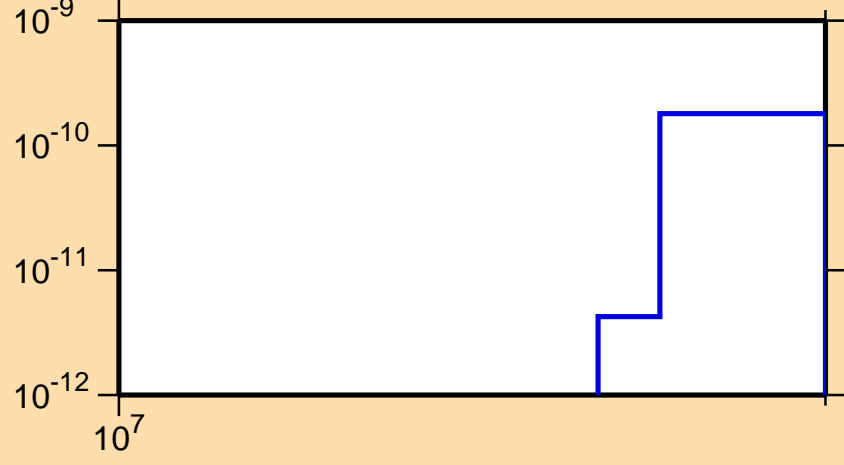
\sigma vs. E for ^{176}\text{Re}(n,\text{pt})
