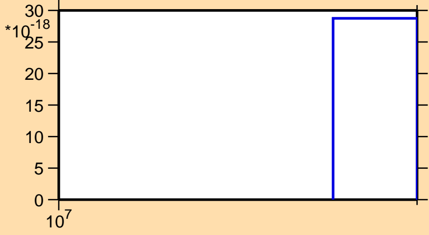
\sigma vs. E for ^{176}\text{Re}(\text{mt } 42)
