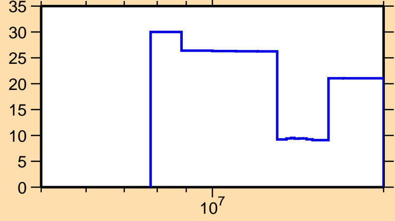
\Delta\sigma/\sigma vs. E for ^{176}\text{Re}(n,2n)
