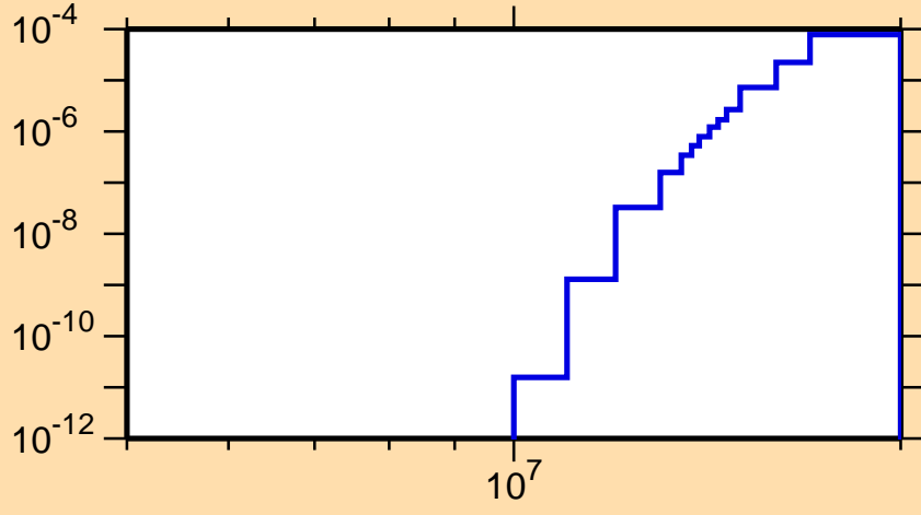
\sigma vs. E for ^{176}\text{Re}(n,2n\alpha)
