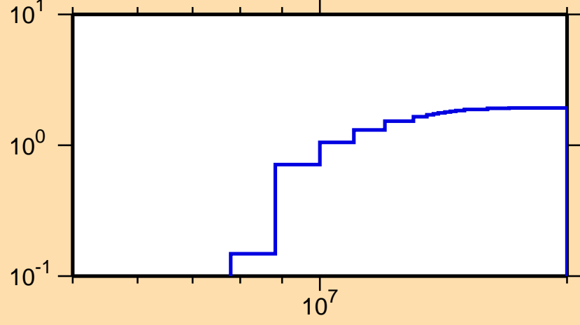
\sigma vs. E for ^{176}\text{Re}(n,2n)
