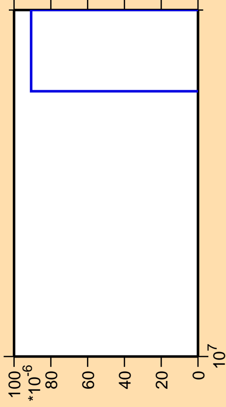
\Delta\sigma/\sigma vs. E for ^{176}\text{Re}(\text{mt } 42)
