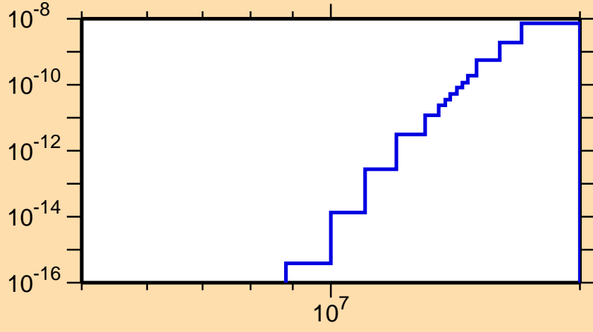
\sigma vs. E for ^{176}\text{Re}(\text{mt117})
