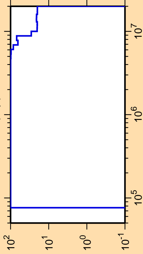
\Delta\sigma/\sigma vs. E for ^{176}\text{Re}(n,p)
