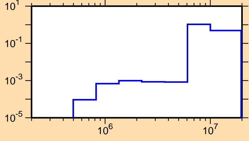
\sigma vs. E for ^{176}\text{Re}(n,n\text{cont.})
