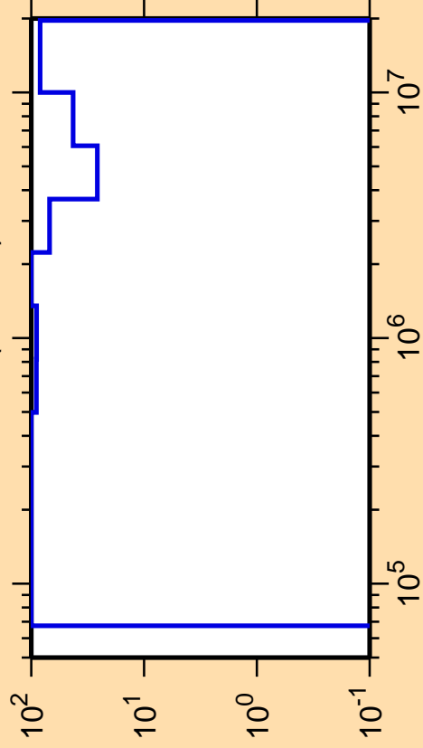
\Delta\sigma/\sigma vs. E for ^{176}\text{Re}(n,\text{inel.})
