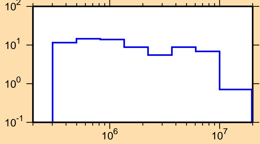
\Delta\sigma/\sigma vs. E for ^{176}\text{Re}(n,\text{tot.})
