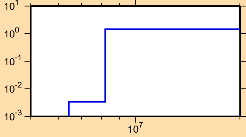
\sigma vs. E for ^{176}\text{Re}(n,2n)
