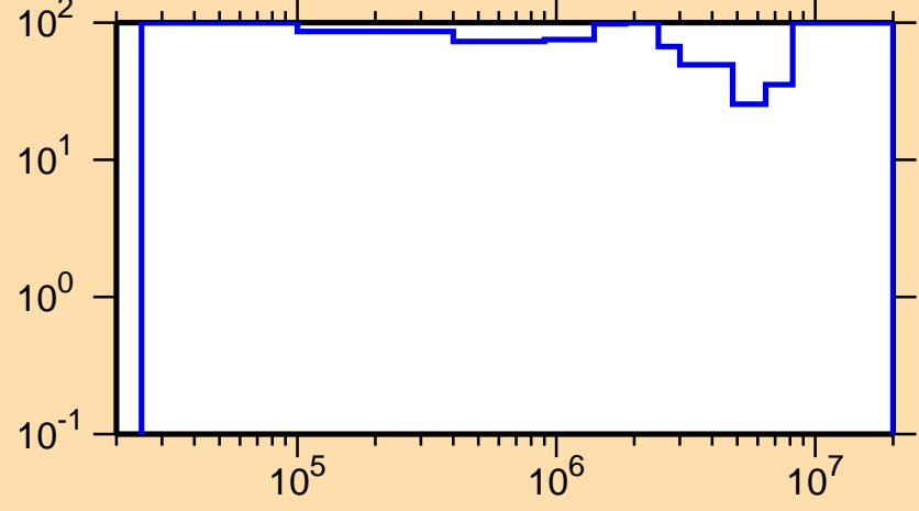
\Delta\sigma/\sigma vs. E for ^{176}\text{Re}(n,n_1)
