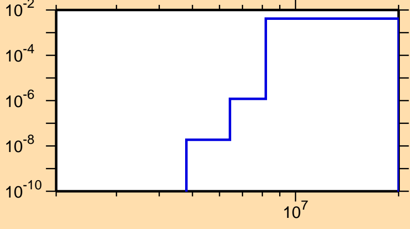
\sigma vs. E for ^{176}\text{Re}(n,d)
