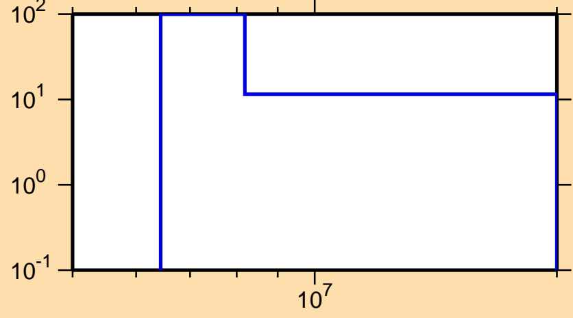
\Delta\sigma/\sigma vs. E for ^{176}\text{Re}(n,2n)
