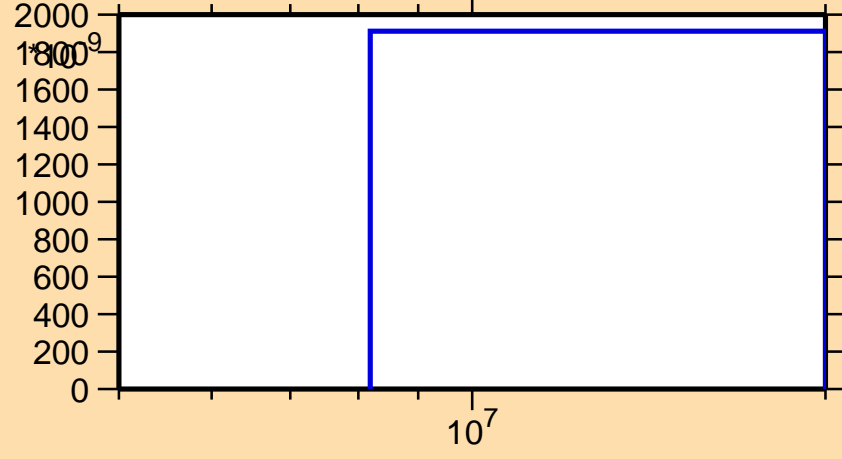
\sigma vs. E for ^{176}\text{Re}(n,\text{nd})
