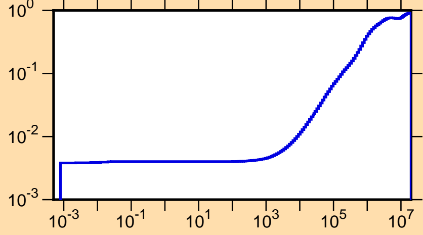
\mu vs. E for ^{177}\text{Re}(\text{mt251})
